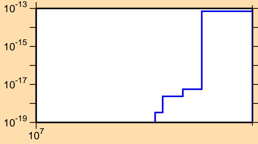
\sigma vs. E for ^{98}\text{Tc} (mt 34)
