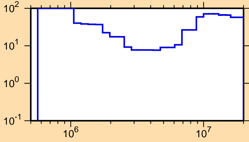
\Delta\sigma/\sigma vs. E for ^{98}\text{Tc}(n,n\text{cont.})
