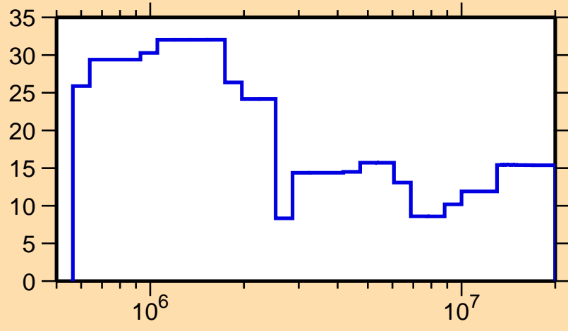
\Delta\sigma/\sigma vs. E for ^{98}\text{Tc}(n, el.)
