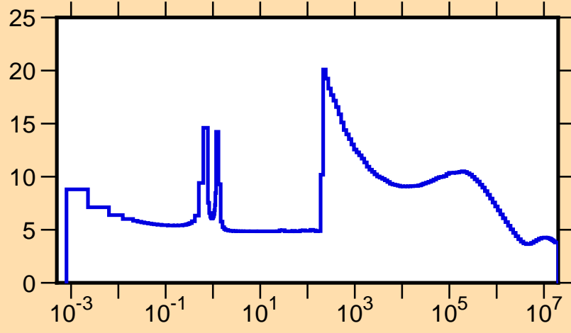
\sigma vs. E for ^{98}\text{Tc}(n,\text{tot.})
