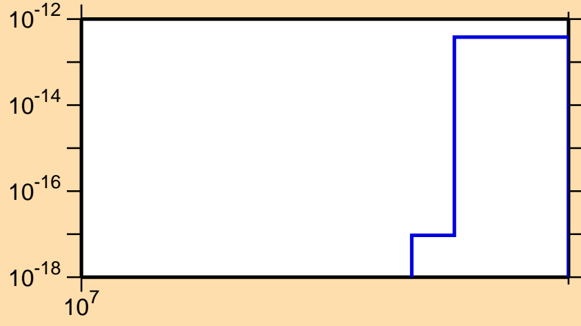
\sigma vs. E for ^{98}\text{Tc}(n,\text{pd})
