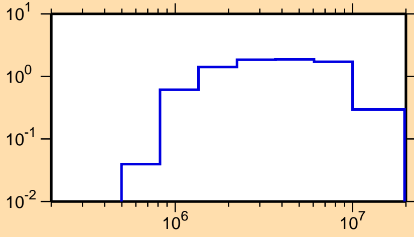
\sigma vs. E for ^{98}\text{Tc}(n,n\text{cont.})
