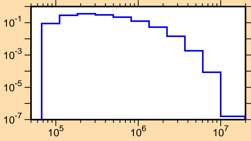
\sigma vs. E for ^{98}\text{Tc}(n,n_4)
