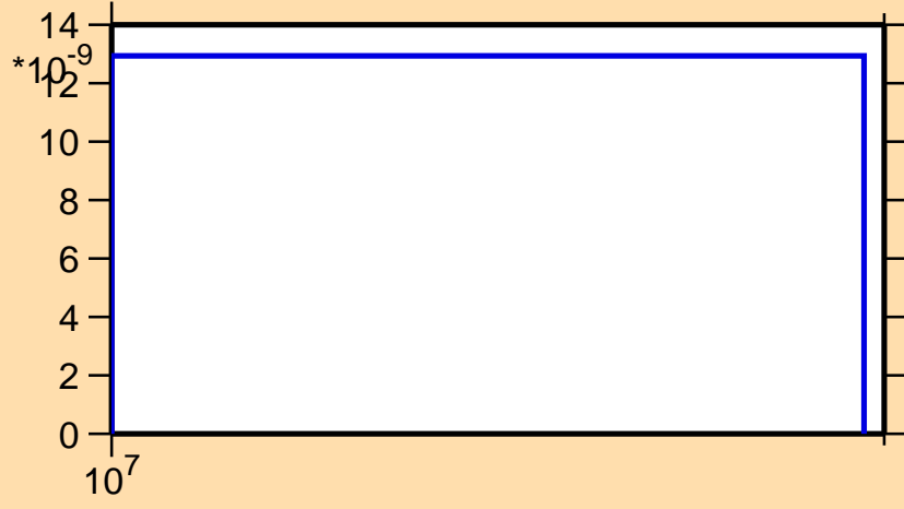
\sigma vs. E for ^{98}\text{Tc}(n,nt)
