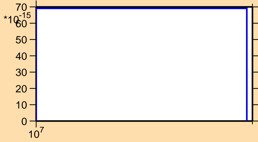
\sigma vs. E for ^{98}\text{Tc} (mt 45)
