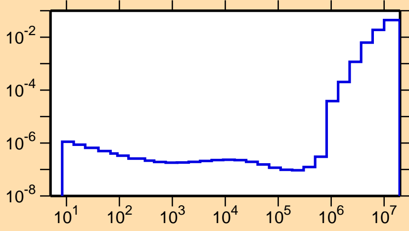
\sigma vs. E for ^{98}\text{Tc}(n,p)
