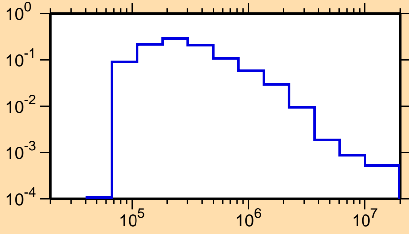
\sigma vs. E for ^{98}\text{Tc}(n,n_2)
