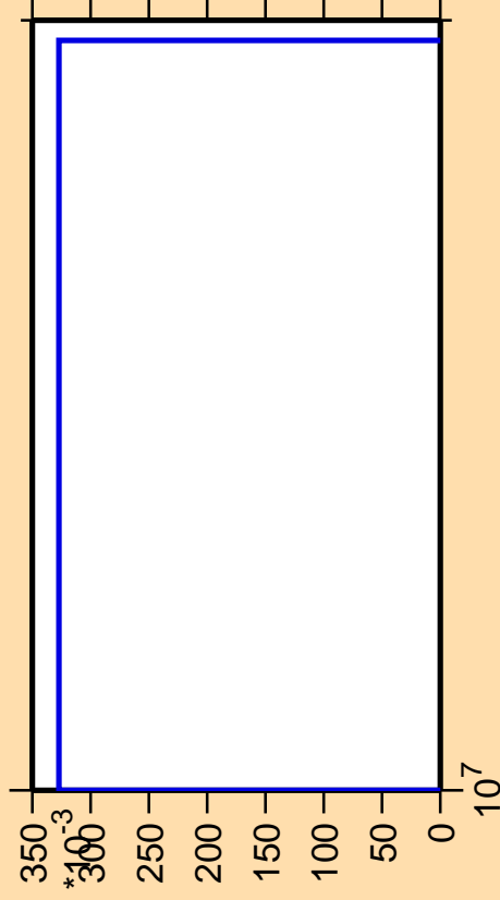
\Delta\sigma/\sigma vs. E for ^{98}\text{Tc} (mt 45)
