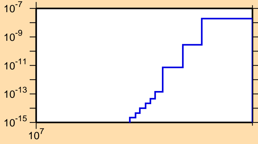
\sigma vs. E for ^{99}\text{Tc}(n,\text{He3})
