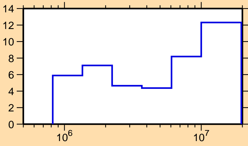
\Delta\sigma/\sigma vs. E for ^{99}\text{Tc}(n,el.)
