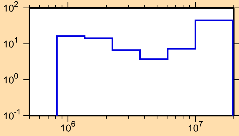
\Delta\sigma/\sigma vs. E for ^{99}\text{Tc}(n,n\text{cont.})
