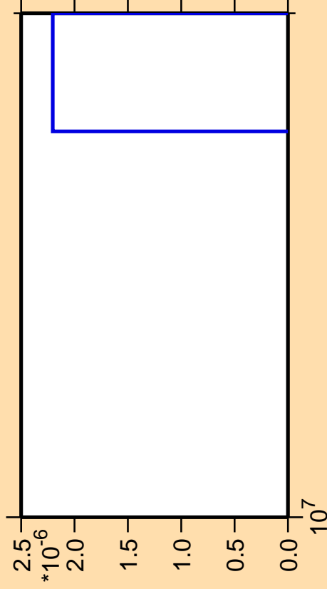
\Delta\sigma/\sigma vs. E for ^{100}\text{Tc} (mt 11)
