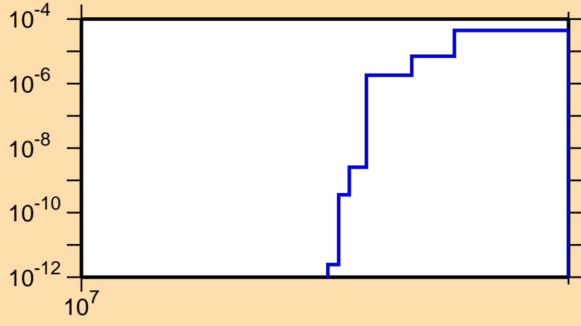
\sigma vs. E for ^{100}\text{Tc}(n,2np)
