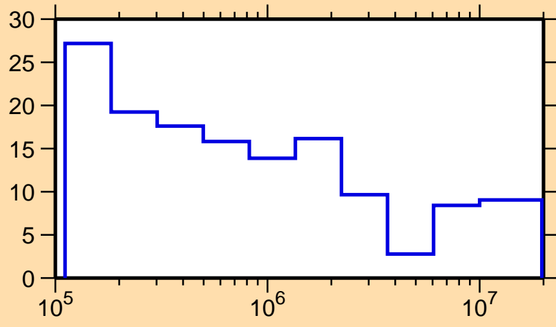
\Delta\sigma/\sigma vs. E for ^{100}\text{Tc}(n,\text{el.})
