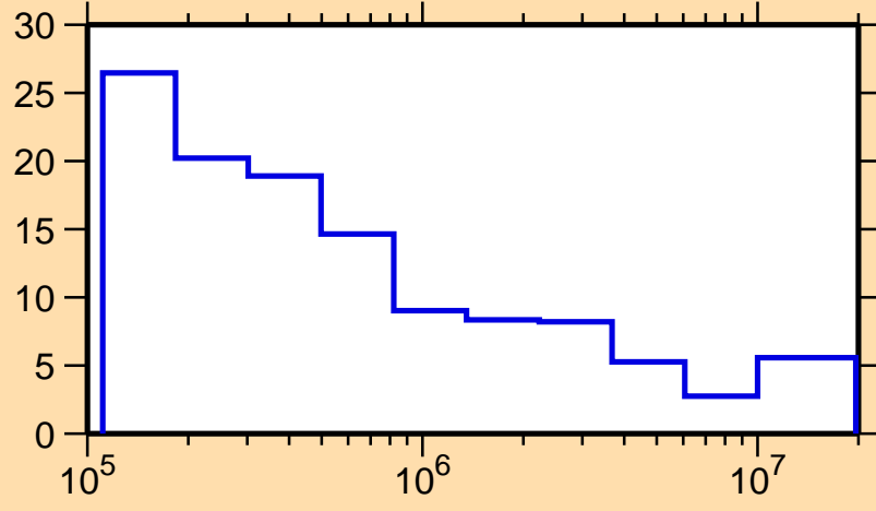
\Delta\sigma/\sigma vs. E for ^{100}\text{Tc}(n,\text{tot.})
