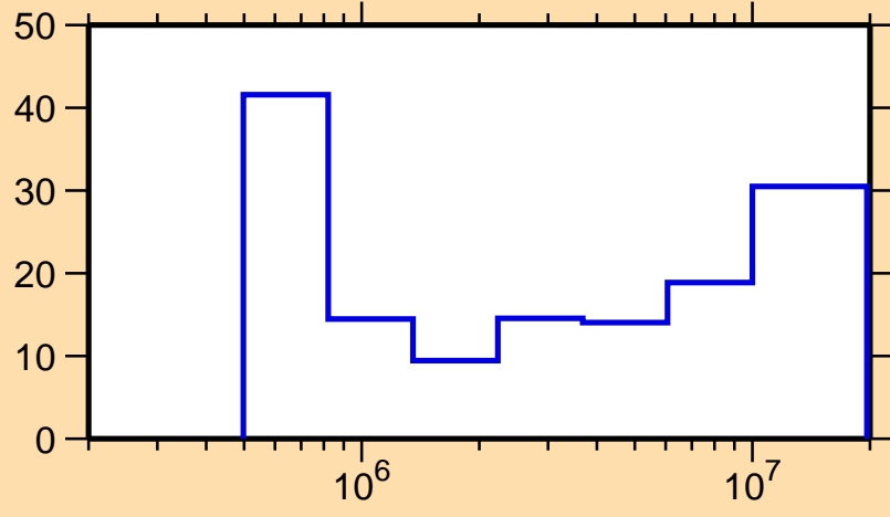
\Delta\sigma/\sigma vs. E for ^{100}\text{Tc}(n,n\text{cont.})
