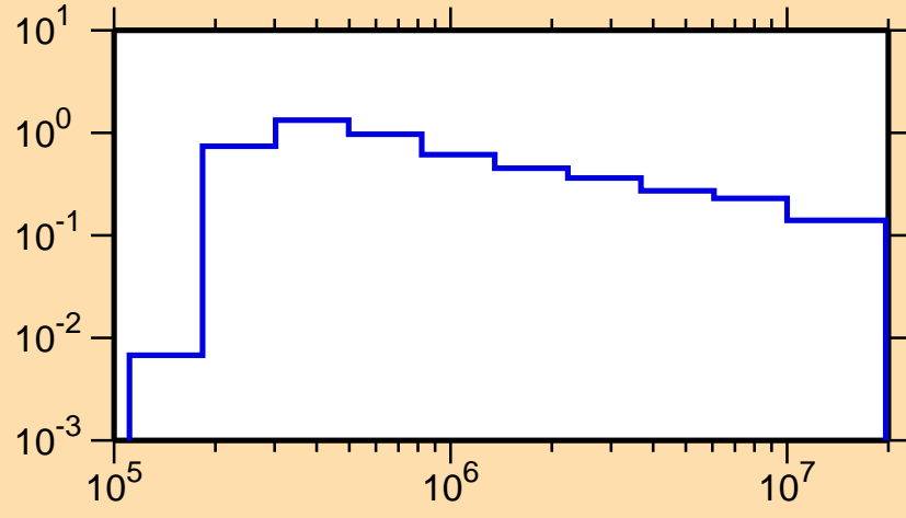
\sigma vs. E for ^{100}\text{Tc}(n,n_1)
