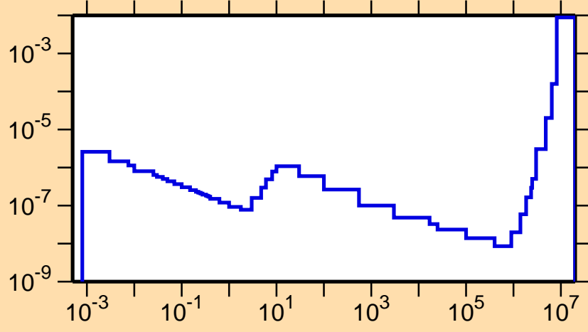
\sigma vs. E for ^{100}\text{Tc}(n,\alpha)
