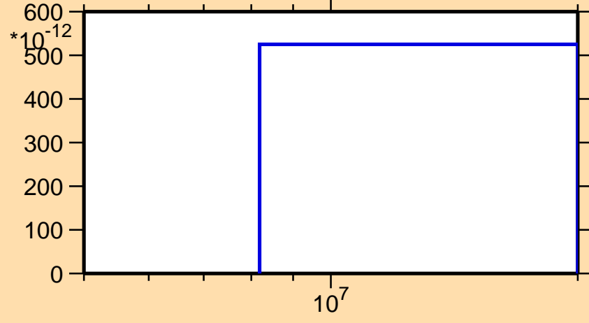
\sigma vs. E for ^{100}\text{Tc}(n,p\alpha)
