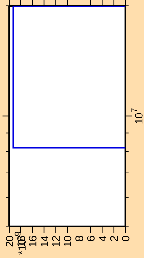
\Delta\sigma/\sigma vs. E for ^{101}\text{Tc}(\text{mt } 11)
