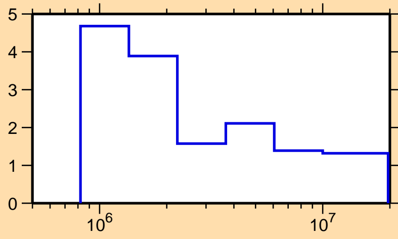
\Delta\sigma/\sigma vs. E for ^{102}\text{Tc}(n,n\text{onel.})
