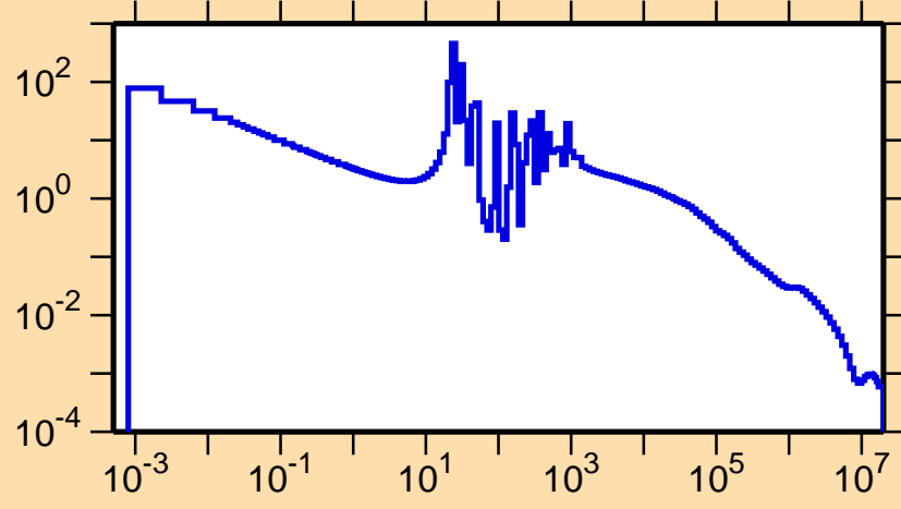
\sigma vs. E for ^{103}\text{Tc}(n,\gamma)
