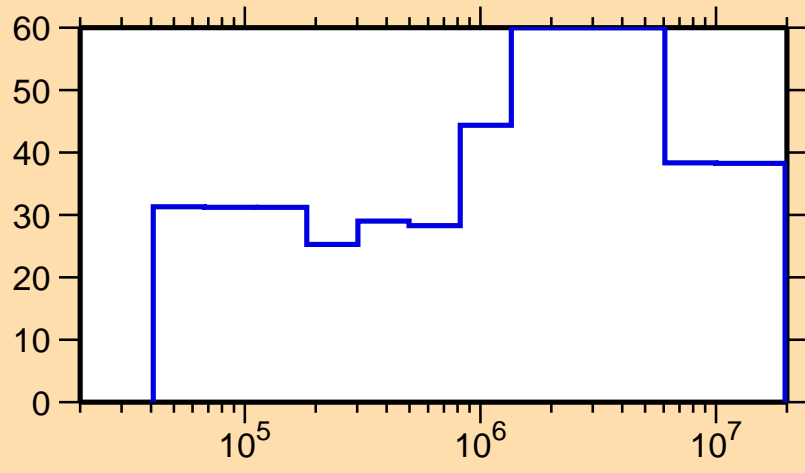
\Delta\sigma/\sigma vs. E for ^{103}\text{Tc}(n,n_1)
