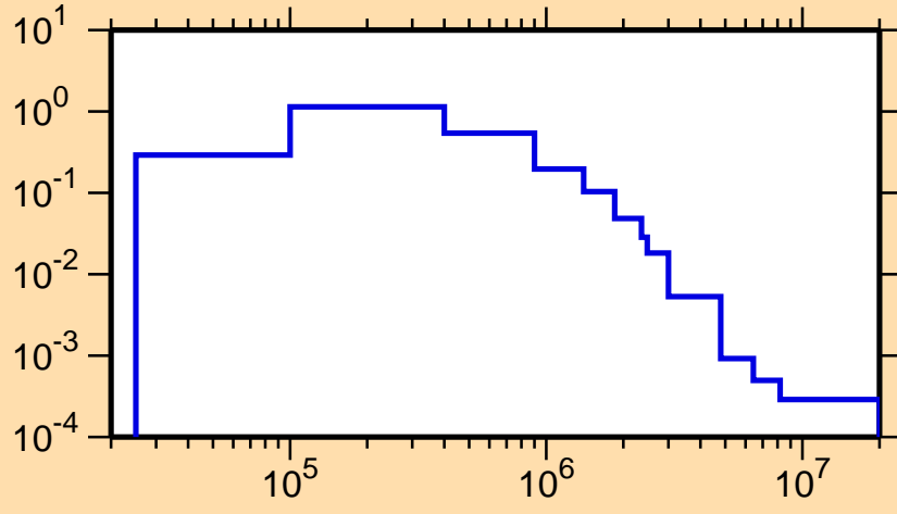
\sigma vs. E for ^{103}\text{Tc}(n,n_1)
