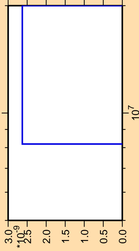
\Delta\sigma/\sigma vs. E for ^{103}\text{Tc} (mt 11)
