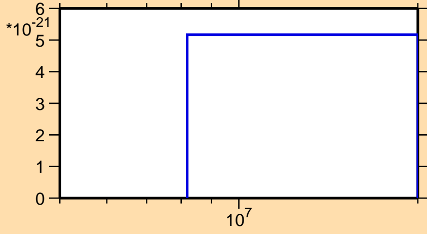
\sigma vs. E for ^{103}\text{Tc} (mt 11)
