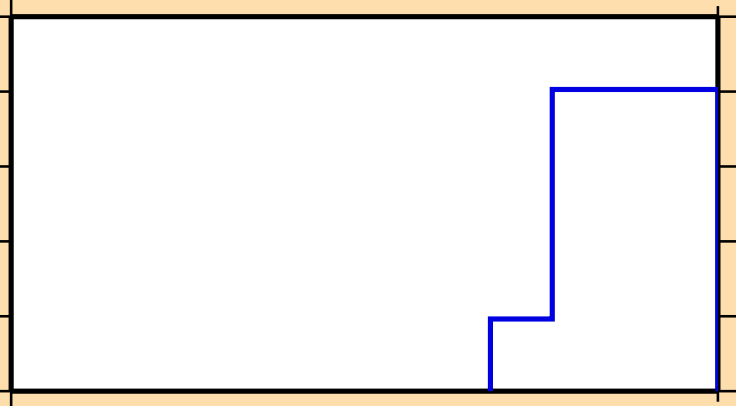
\sigma vs. E for ^{104}\text{Tc}(n,nt)
