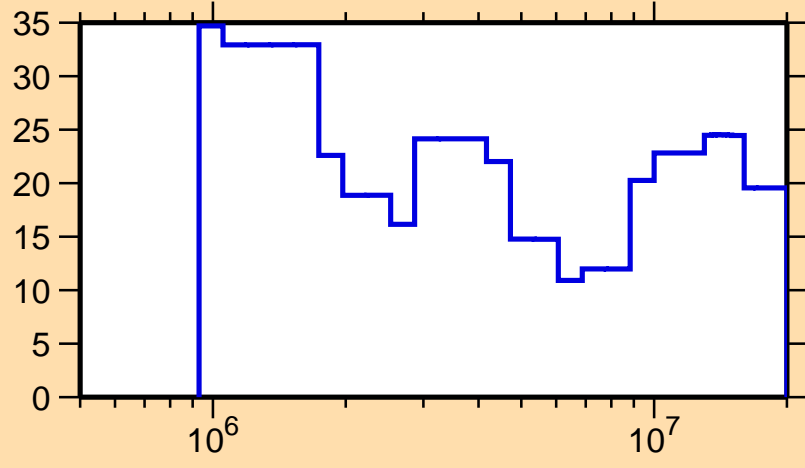
\Delta\sigma/\sigma vs. E for ^{104}\text{Tc}(n, el.)
