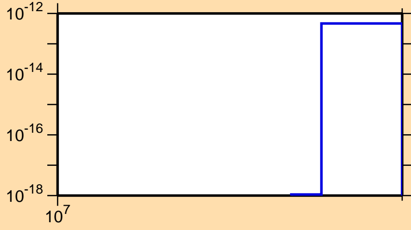
\sigma vs. E for ^{104}\text{Tc}(n,\text{He3})
