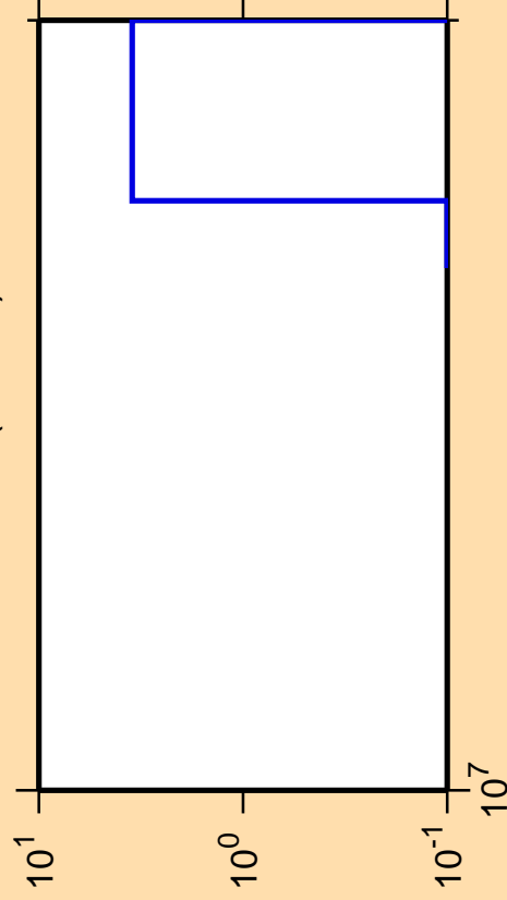
\Delta\sigma/\sigma vs. E for ^{104}\text{Tc}(n,\text{He3})
