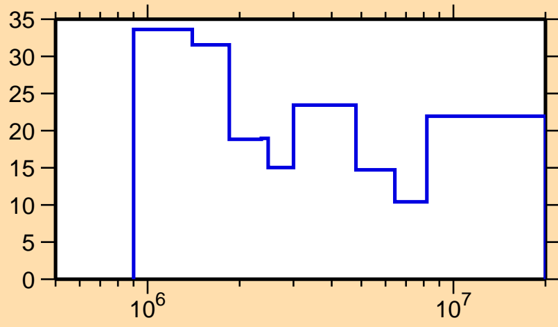
\Delta\sigma/\sigma vs. E for ^{104}\text{Tc}(n, el.)
