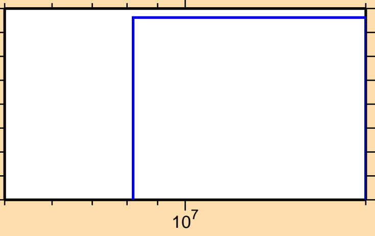
\sigma vs. E for ^{104}\text{Tc}(n,\text{He3})
