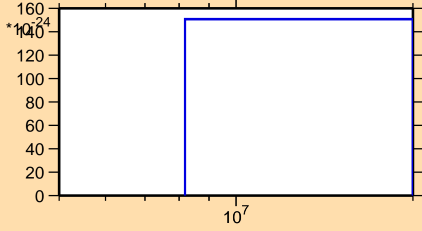
\sigma vs. E for ^{104}\text{Tc} (mt 34)
