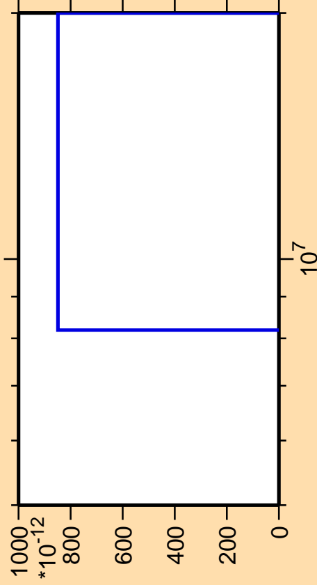
\Delta\sigma/\sigma vs. E for ^{104}\text{Tc} (mt 34)
