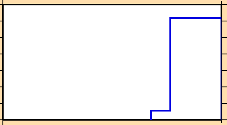
\sigma vs. E for ^{105}\text{Tc}(n,2n\alpha)
