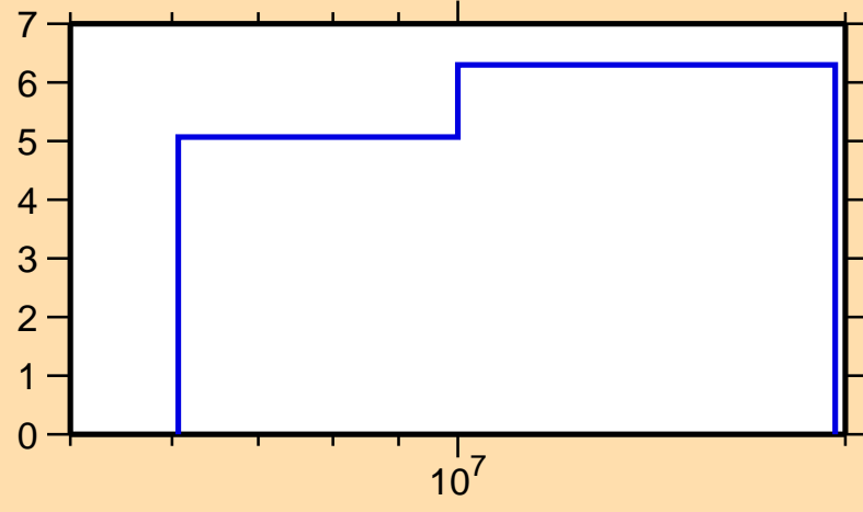
\Delta\sigma/\sigma vs. E for ^{105}\text{Tc}(n,\text{el.})
