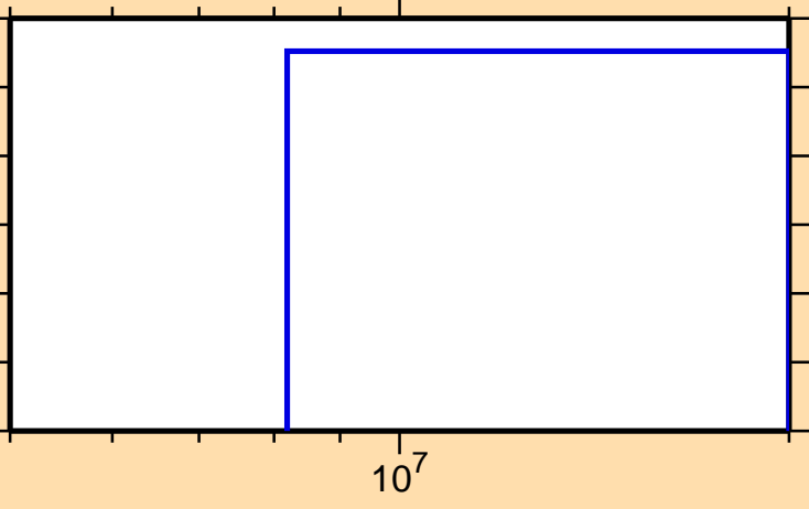
\sigma vs. E for ^{105}\text{Tc}(n,n\alpha)
