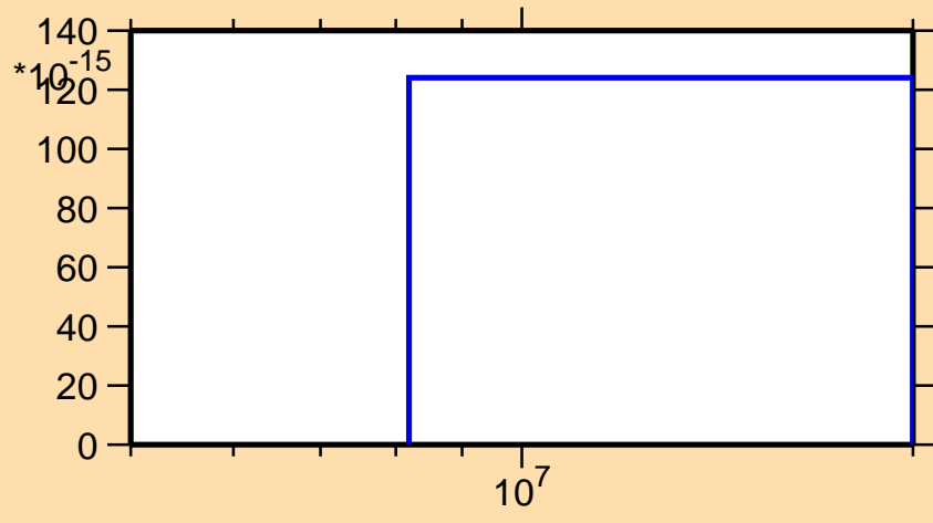
\sigma vs. E for ^{105}\text{Tc}(n,2n\alpha)
