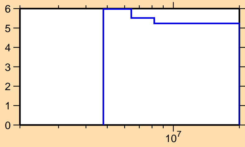
\Delta\sigma/\sigma vs. E for ^{105}\text{Tc}(n,el.)
