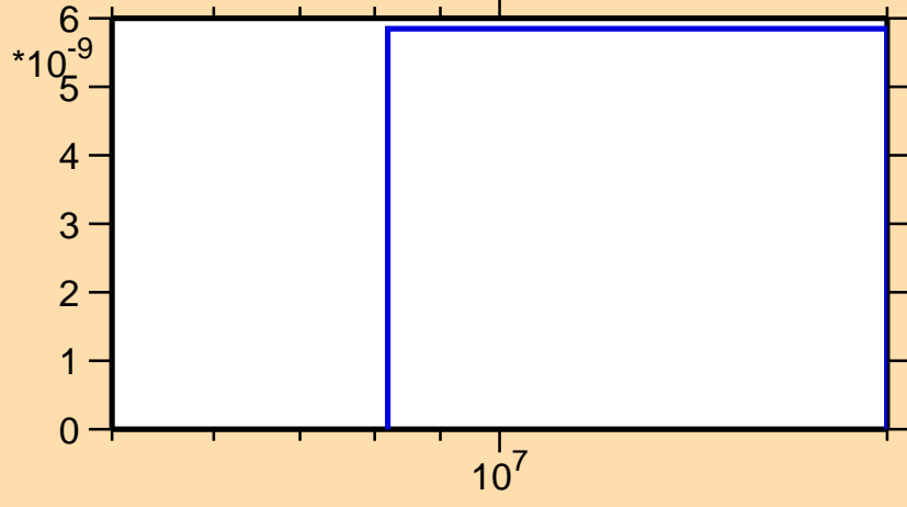
\sigma vs. E for ^{105}\text{Tc}(n,nt)
