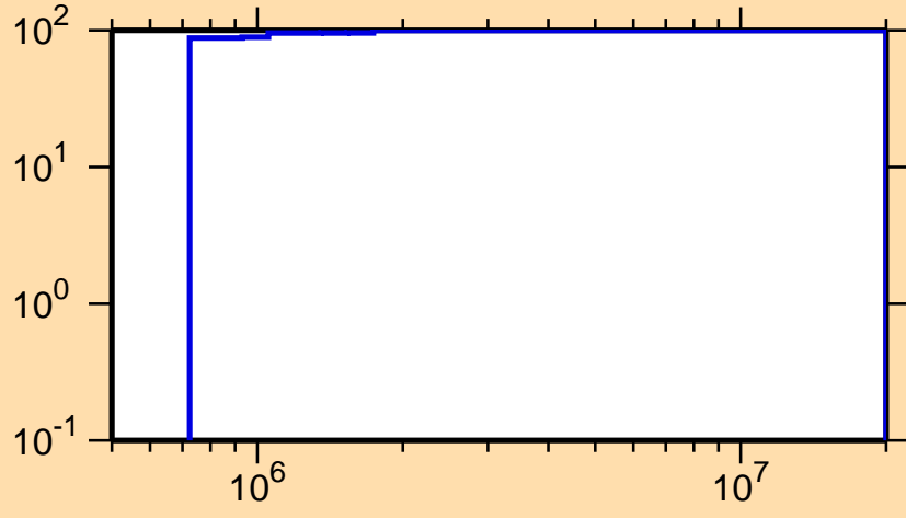
\Delta\sigma/\sigma vs. E for ^{106}\text{Tc}(n,n_1)
