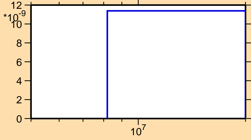
\sigma vs. E for ^{106}\text{Tc}(n,nt)
