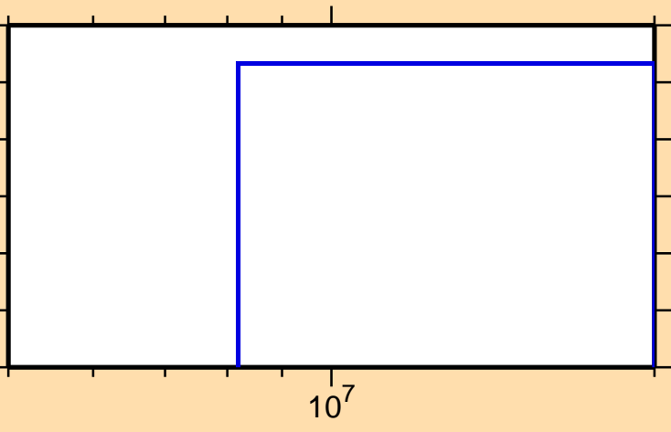
\sigma vs. E for ^{106}\text{Tc}(n,n\alpha)
