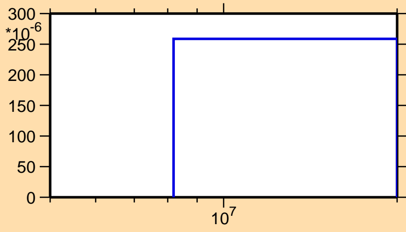
\sigma vs. E for ^{106}\text{Tc}(n,d)
