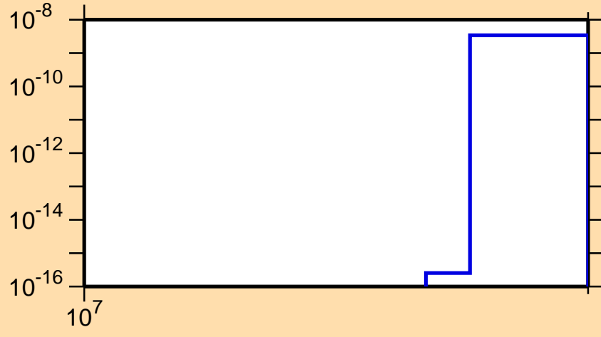
\sigma vs. E for ^{107}\text{Tc}(n,2np)
