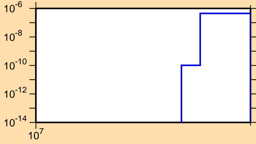
\sigma vs. E for ^{107}\text{Tc}(n,\text{nd})
