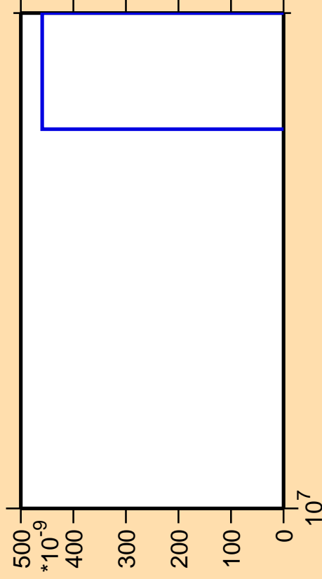
\Delta\sigma/\sigma vs. E for ^{107}\text{Tc} (mt 11)
