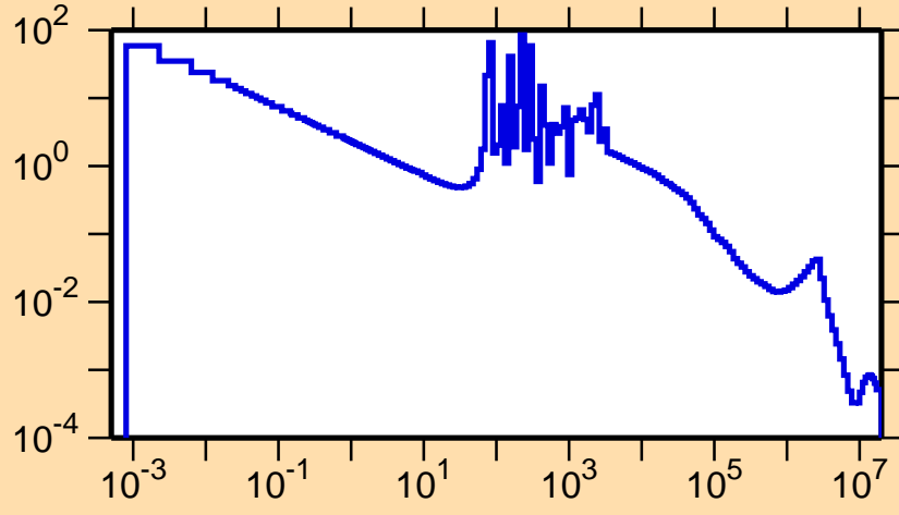
\sigma vs. E for ^{107}\text{Tc}(n,\gamma)
