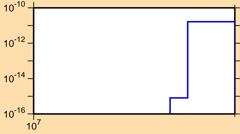
\sigma vs. E for ^{107}\text{Tc}(n,2n\alpha)
