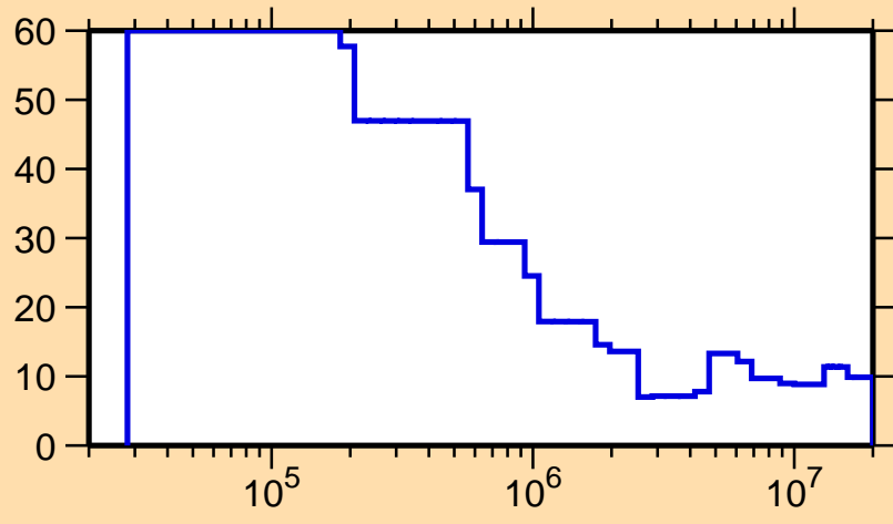
\Delta\sigma/\sigma vs. E for ^{107}\text{Tc}(n,\text{nonel.})
