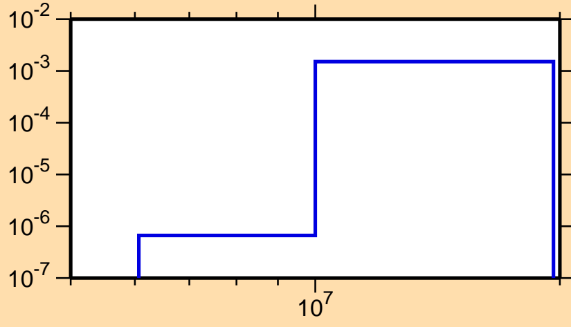
\sigma vs. E for ^{107}\text{Tc}(n,p)
