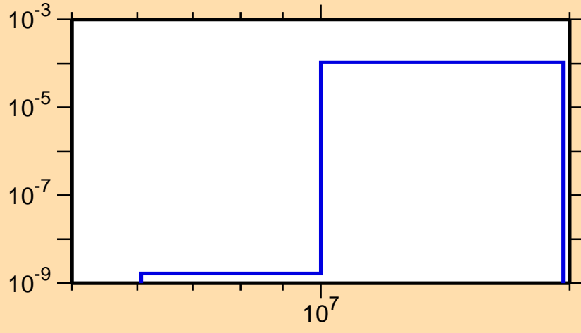
\sigma vs. E for ^{107}\text{Tc}(n,\alpha)
