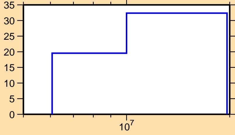
\Delta\sigma/\sigma vs. E for ^{107}\text{Tc}(n,el.)
