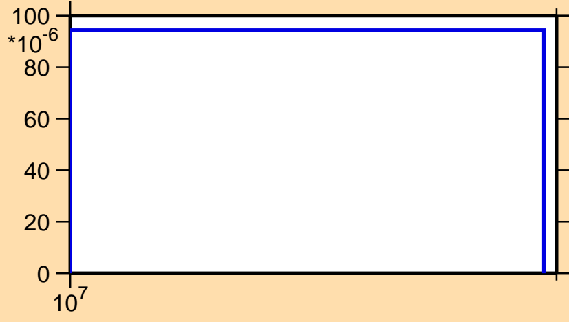
\sigma vs. E for ^{107}\text{Tc}(n,np)
