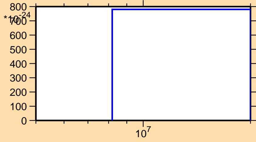
\sigma vs. E for ^{107}\text{Tc} (mt 11)
