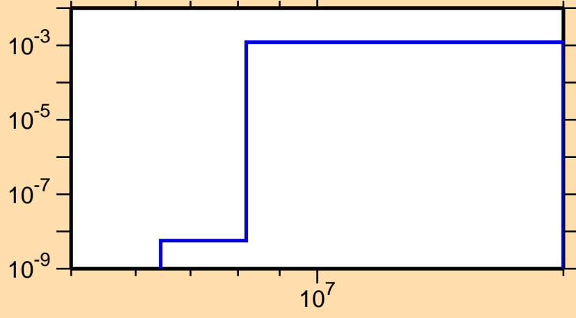
\sigma vs. E for ^{107}\text{Tc}(n,p)
