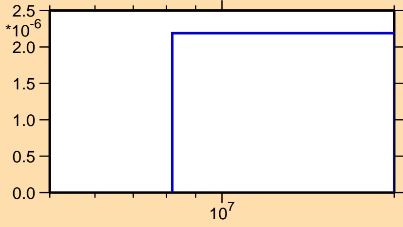
\sigma vs. E for ^{107}\text{Tc}(n,n\alpha)
