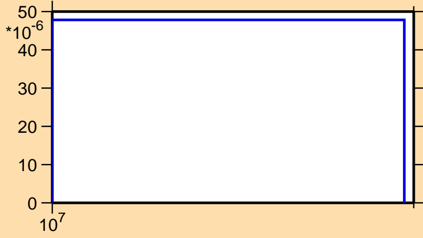
\sigma vs. E for ^{108}\text{Tc}(n,np)
