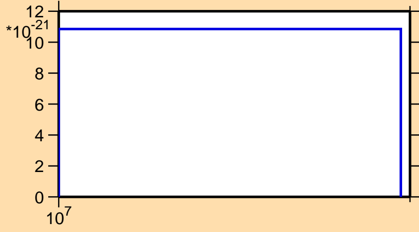
\sigma vs. E for ^{108}\text{Tc}(n,3n\alpha)
