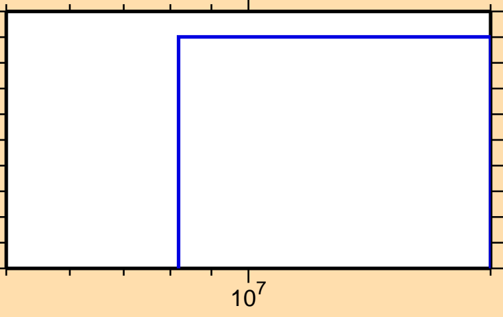
\sigma vs. E for ^{109}\text{Tc}(n,np)
