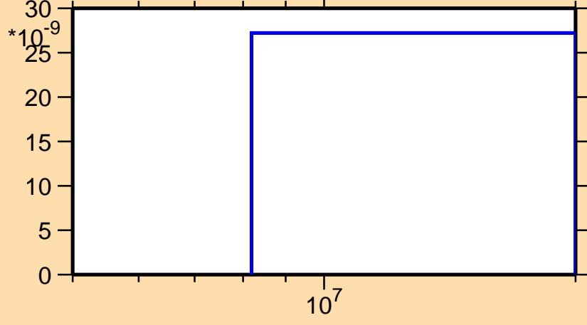
\sigma vs. E for ^{109}\text{Tc}(n,nt)
