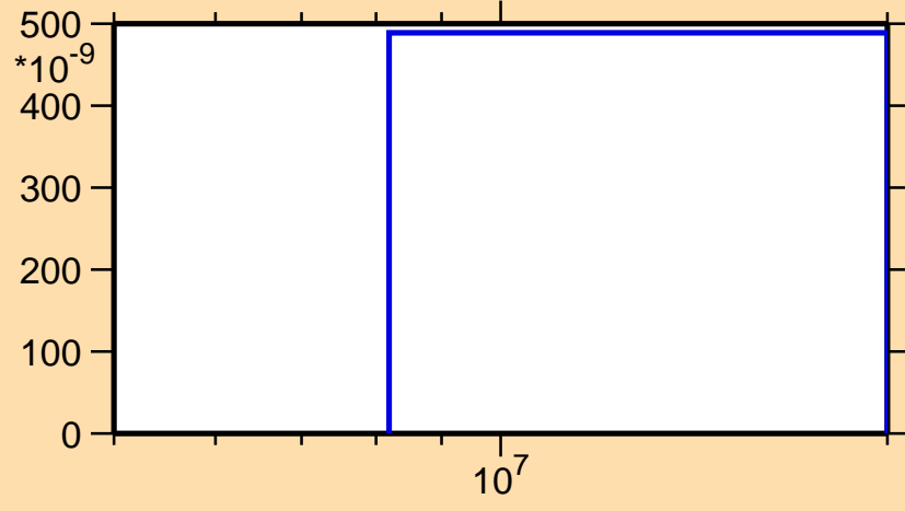
\sigma vs. E for ^{109}\text{Tc}(n,n\alpha)
