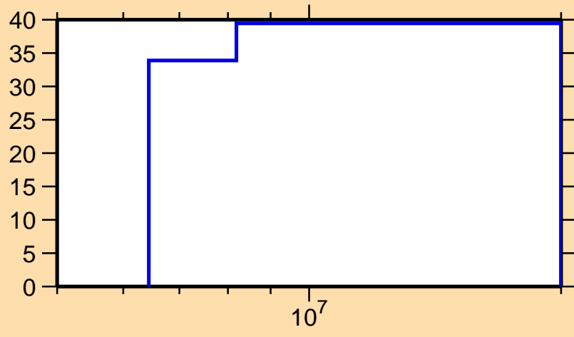
\Delta\sigma/\sigma vs. E for ^{109}\text{Tc}(n,n\text{cont.})
