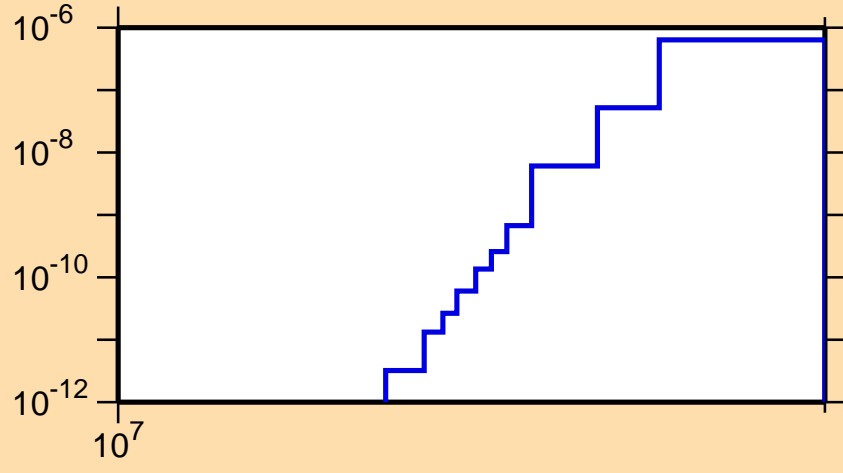
\sigma vs. E for ^{108}\text{Te}(\text{mt } 34)
