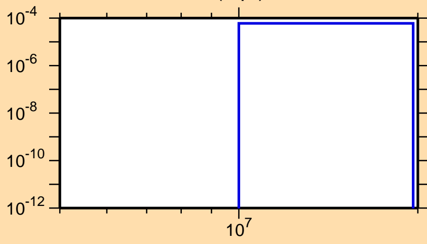
\sigma vs. E for ^{108}\text{Te}(n,pt)
