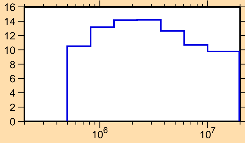
\Delta\sigma/\sigma vs. E for ^{108}\text{Te}(n,\text{nonel.})
