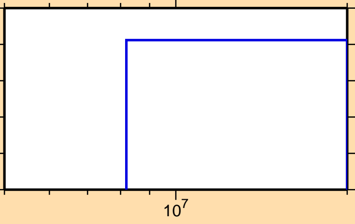
\sigma vs. E for ^{108}\text{Te}(n,2np)
