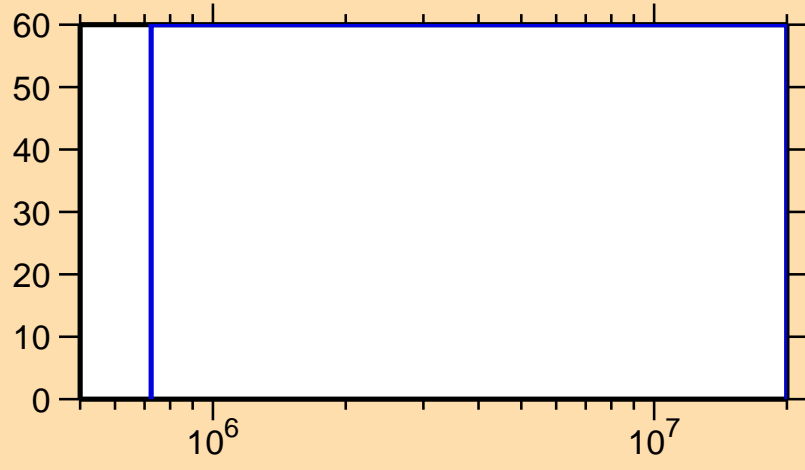
\Delta\sigma/\sigma vs. E for ^{109}\text{Te}(n,n\text{cont.})
