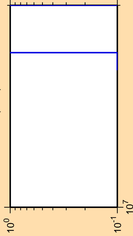
\Delta\sigma/\sigma vs. E for ^{109}\text{Te}(n,nt)
