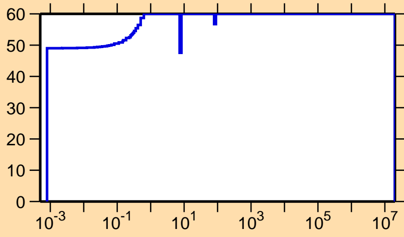
\Delta\sigma/\sigma vs. E for ^{109}\text{Te}(n,\gamma)
