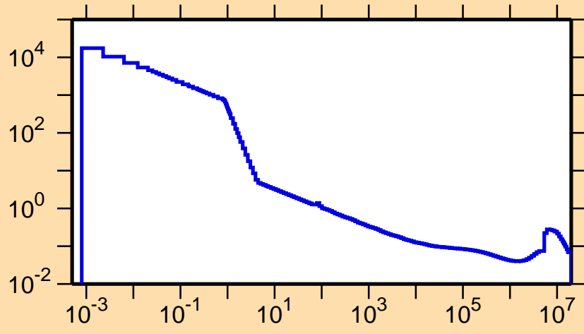
\sigma vs. E for ^{109}\text{Te}(n,\alpha)
