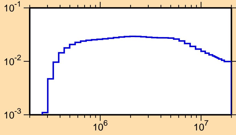
\sigma vs. E for ^{109}\text{Te}(n,n_2)
