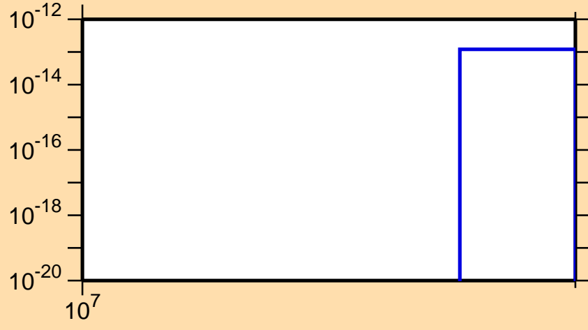
\sigma vs. E for ^{109}\text{Te}(n,nt)
