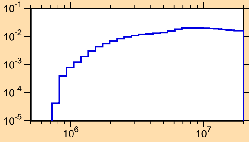
\sigma vs. E for ^{109}\text{Te}(n,n\text{cont.})
