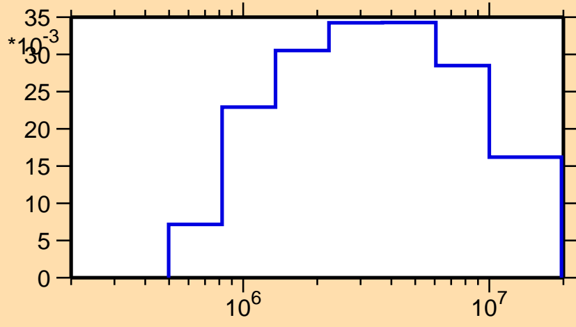
\sigma vs. E for ^{109}\text{Te}(n,n_3)
