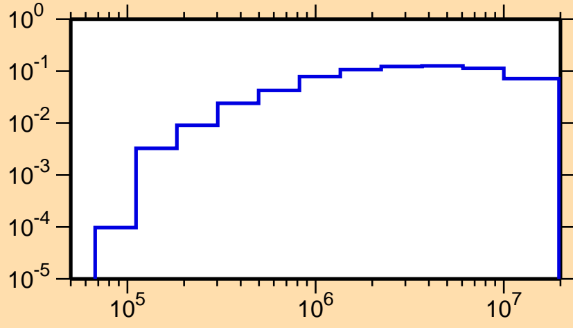
\sigma vs. E for ^{109}\text{Te}(n,\text{inel.})
