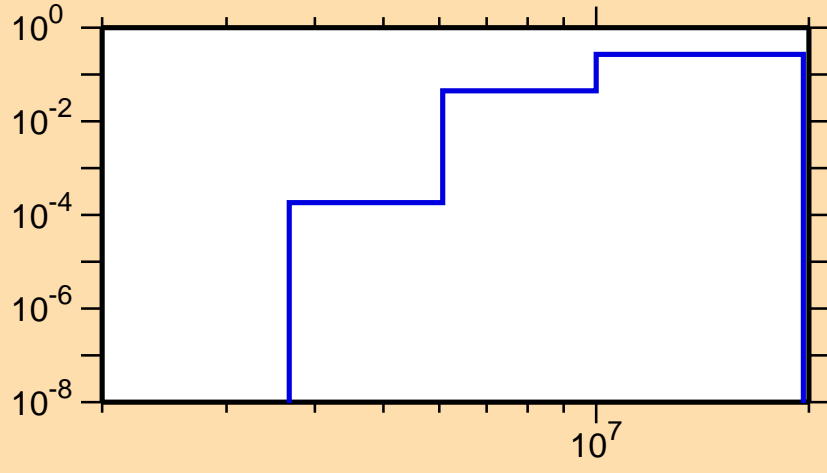
\sigma vs. E for ^{109}\text{Te}(n,np)
