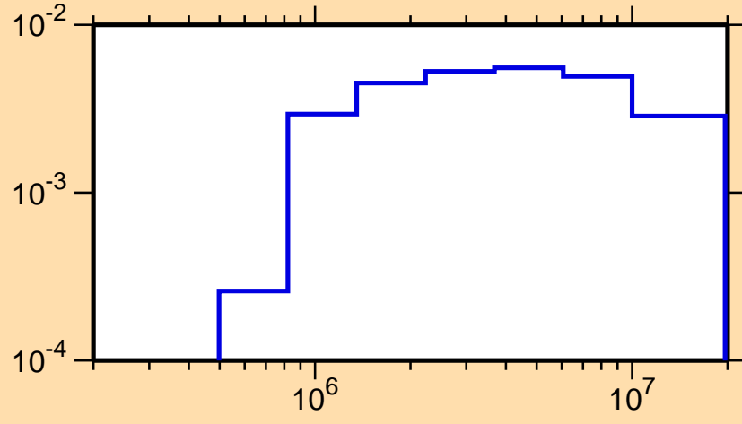
\sigma vs. E for ^{109}\text{Te}(n,n_4)
