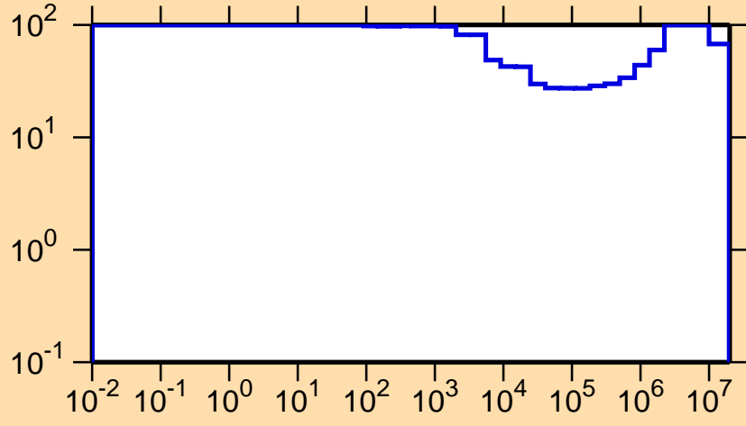
\Delta\sigma/\sigma vs. E for ^{109}\text{Te}(n,p)
