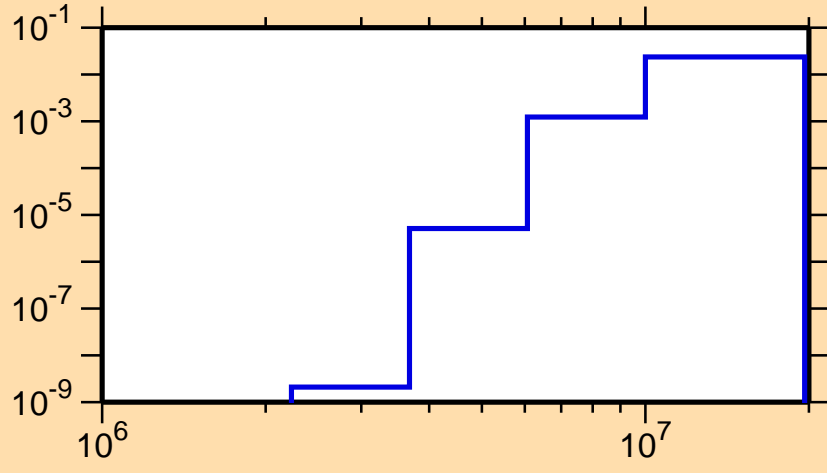
\sigma vs. E for ^{109}\text{Te}(n,d)
