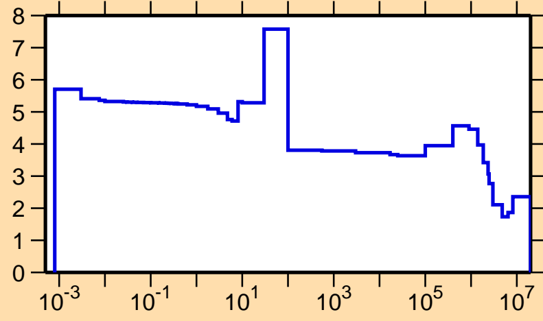
\sigma vs. E for ^{109}\text{Te}(n,\text{el.})
