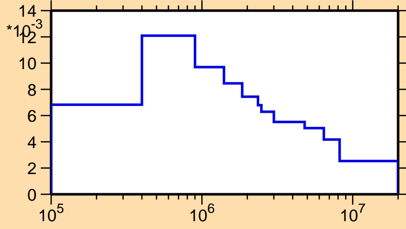
\sigma vs. E for ^{109}\text{Te}(n,n_1)
