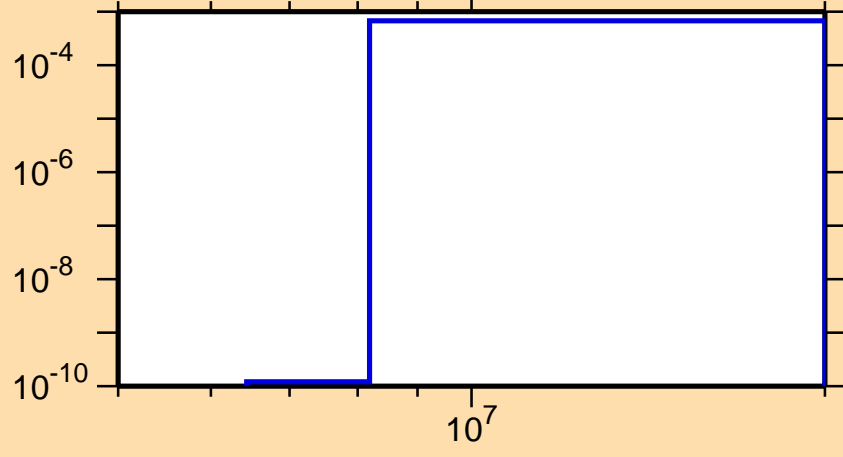
\sigma vs. E for ^{109}\text{Te}(n,t)
