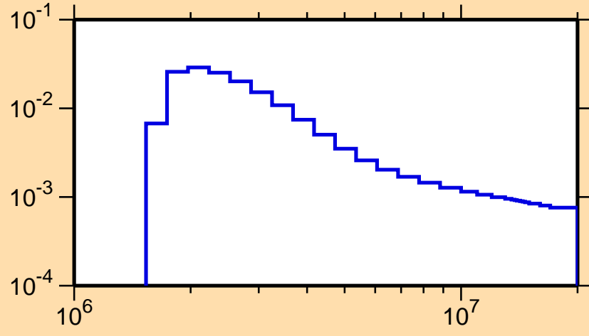
\sigma vs. E for ^{110}\text{Te}(n,n_3)
