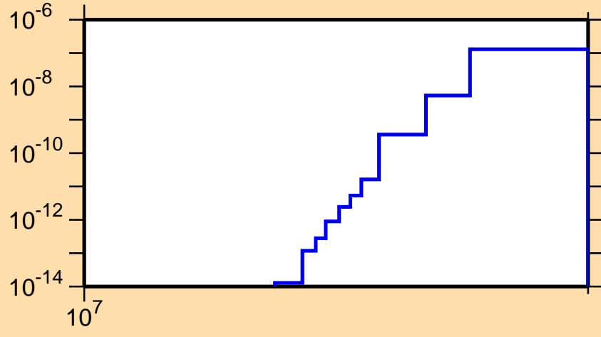
\sigma vs. E for ^{110}\text{Te} (mt 34)
