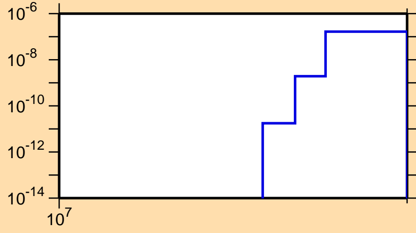
\sigma vs. E for ^{110}\text{Te}(n,\text{nd})
