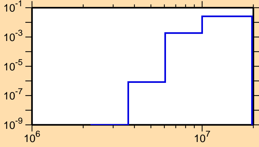
\sigma vs. E for ^{110}\text{Te}(n,n\alpha)
