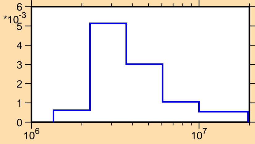
\sigma vs. E for ^{110}\text{Te}(n,n_4)
