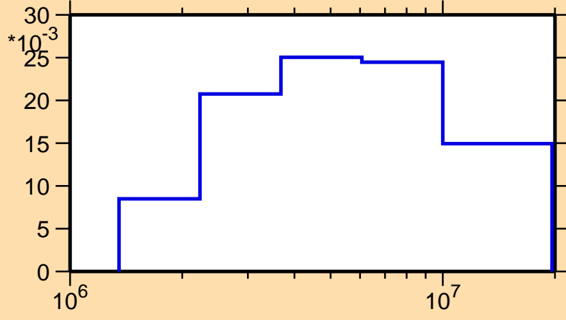
\sigma vs. E for ^{110}\text{Te}(n,n_2)
