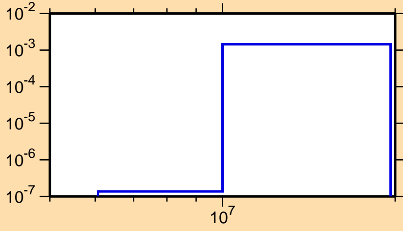
\sigma vs. E for ^{110}\text{Te}(n,pd)
