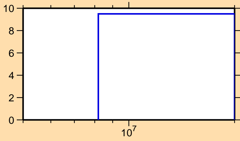
\Delta\sigma/\sigma vs. E for ^{110}\text{Te}(n,\text{nonel.})
