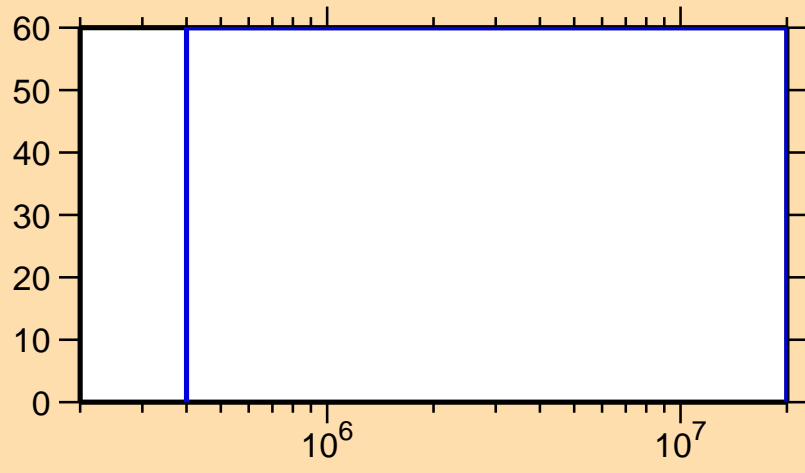
\Delta\sigma/\sigma vs. E for ^{110}\text{Te}(n,\text{inel.})
