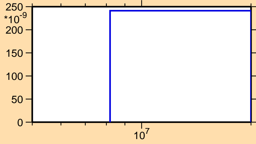
\sigma vs. E for ^{110}\text{Te}(\text{mt117})
