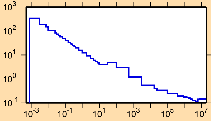
\sigma vs. E for ^{110}\text{Te}(n,\alpha)
