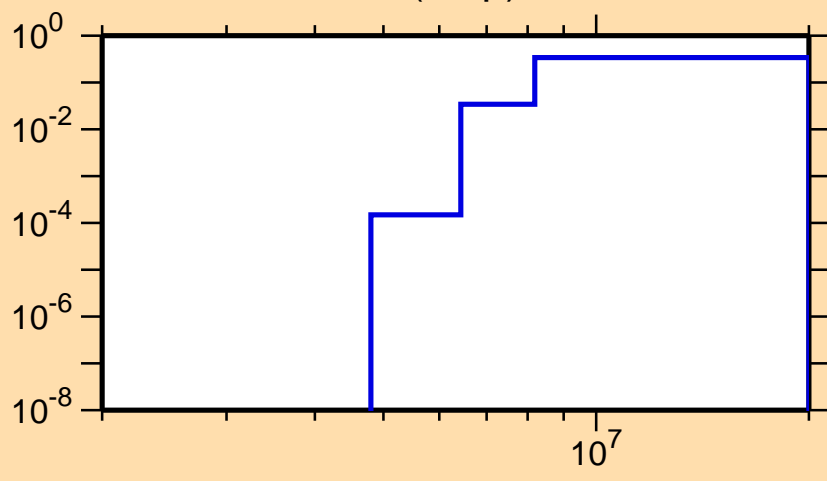
\sigma vs. E for ^{110}\text{Te}(n,np)
