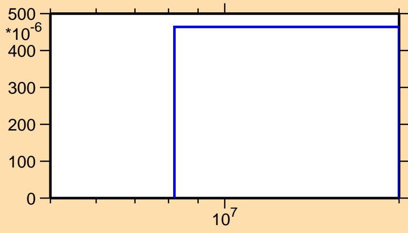
\sigma vs. E for ^{110}\text{Te}(n,2n)
