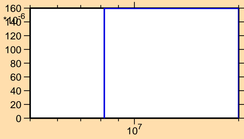
\sigma vs. E for ^{110}\text{Te}(n,t)
