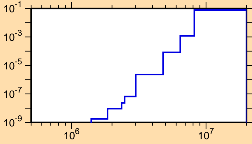
\sigma vs. E for ^{110}\text{Te}(n,p\alpha)
