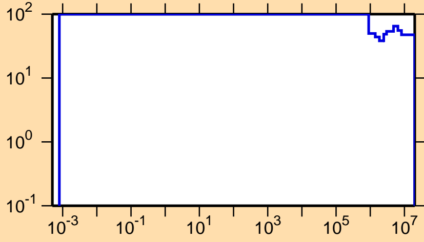
\Delta\sigma/\sigma vs. E for ^{110}\text{Te}(n,p)
