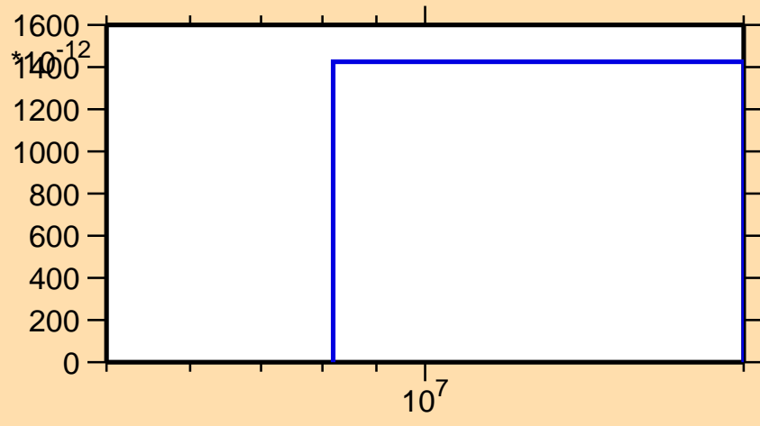
\sigma vs. E for ^{110}\text{Te}(n,nd)
