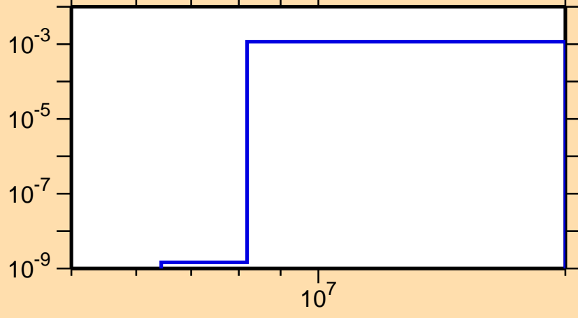
\sigma vs. E for ^{110}\text{Te}(n,pd)
