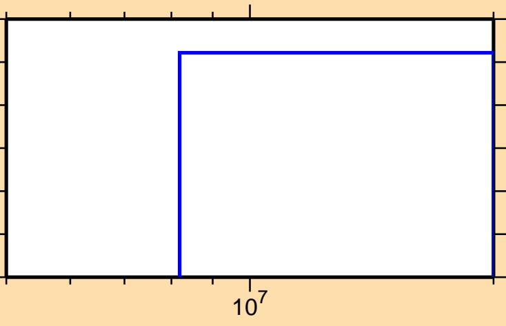
\sigma vs. E for ^{110}\text{Te}(n,2np)
