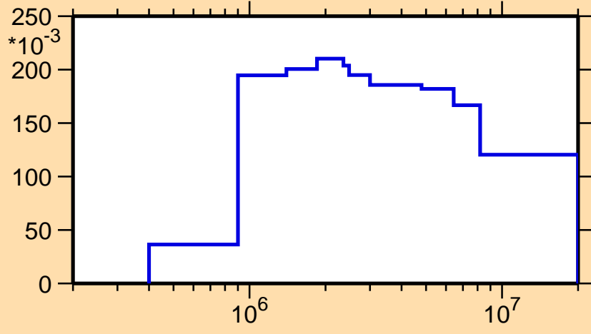
\sigma vs. E for ^{110}\text{Te}(n,\text{inel.})
