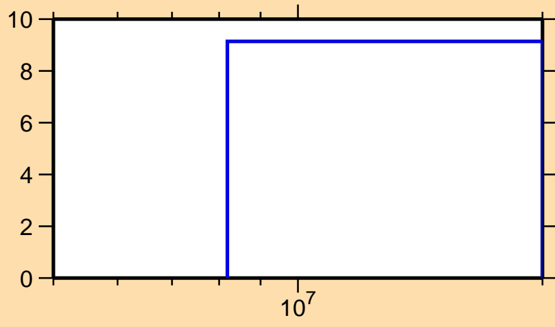
\Delta\sigma/\sigma vs. E for ^{110}\text{Te}(n,\text{tot.})
