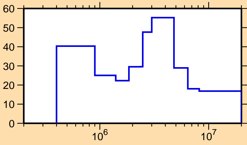
\Delta\sigma/\sigma vs. E for ^{110}\text{Te}(n,\text{el.})
