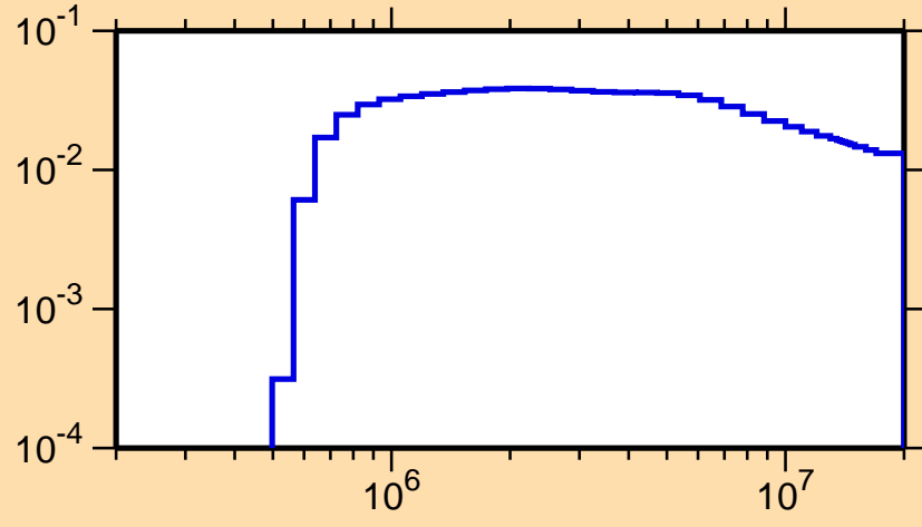
\sigma vs. E for ^{111}\text{Te}(n,n_2)
