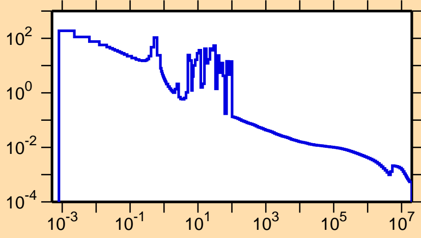
\sigma vs. E for ^{111}\text{Te}(n,\gamma)
