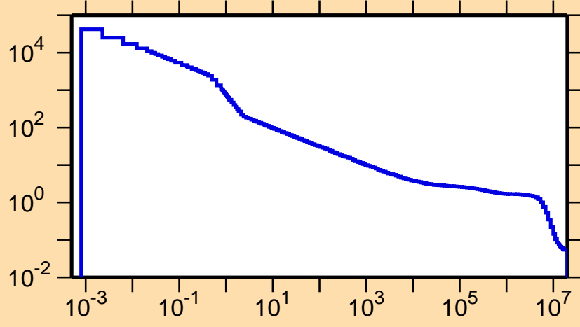
\sigma vs. E for ^{111}\text{Te}(n,p)
