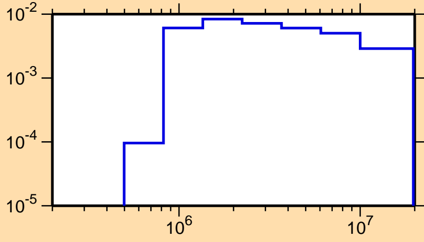
\sigma vs. E for ^{111}\text{Te}(n,n_3)
