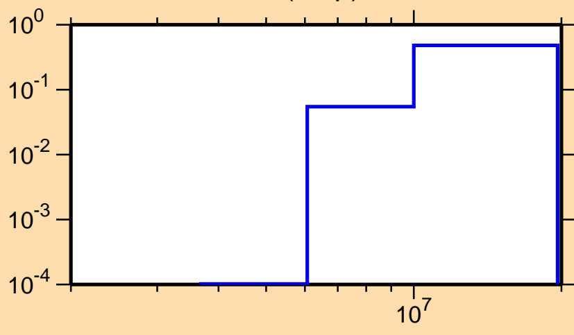
\sigma vs. E for ^{111}\text{Te}(n,np)
