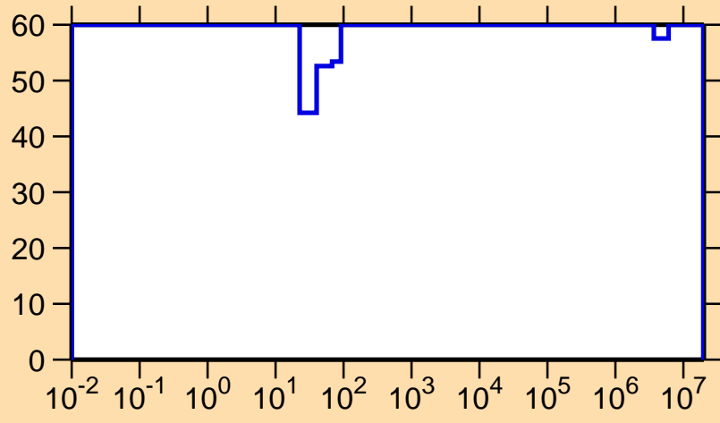
\Delta\sigma/\sigma vs. E for ^{111}\text{Te}(n,\gamma)
