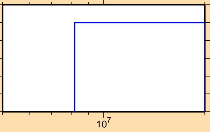
\sigma vs. E for ^{111}\text{Te}(n,2n)
