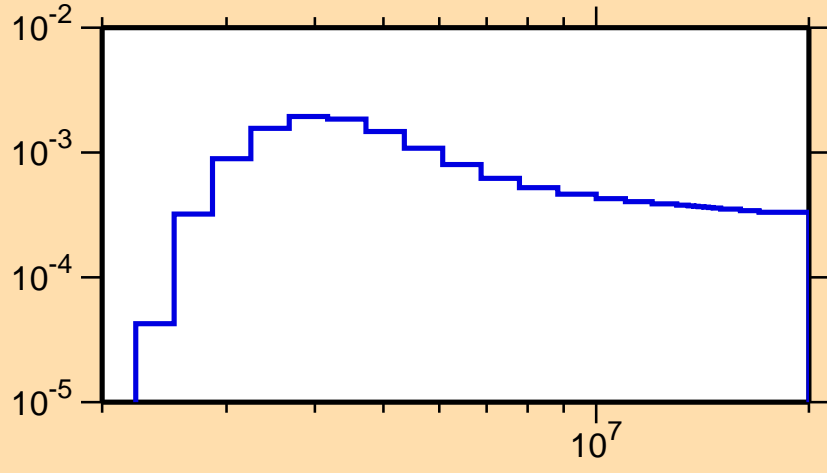
\sigma vs. E for ^{112}\text{Te}(n,n_3)
