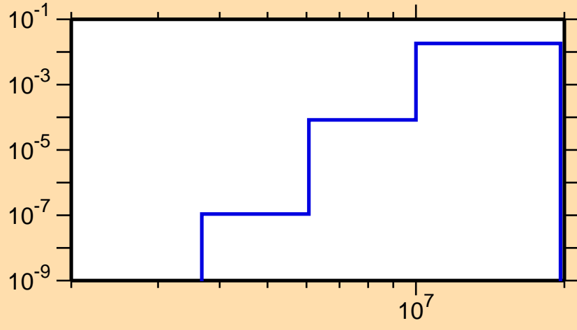
\sigma vs. E for ^{112}\text{Te}(n,p\alpha)
