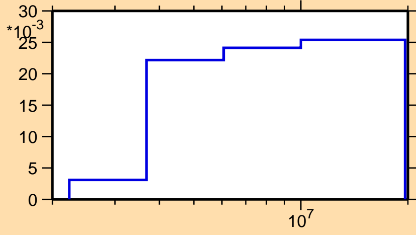
\sigma vs. E for ^{112}\text{Te}(n,n_4)
