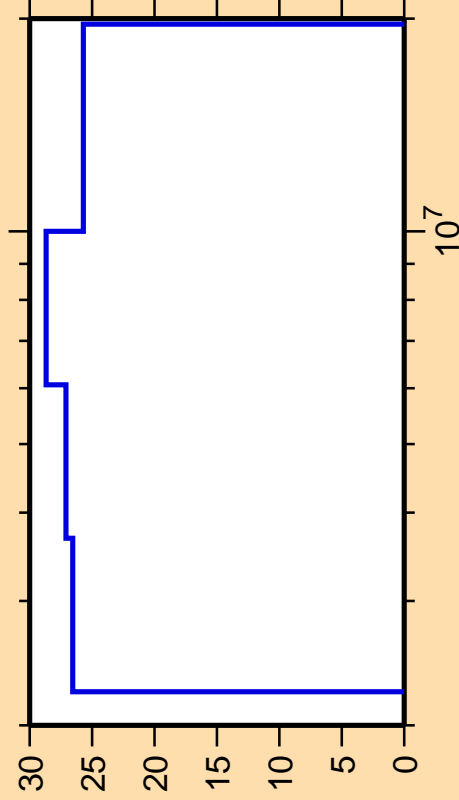
\Delta\sigma/\sigma vs. E for ^{112}\text{Te}(n,n_4)
