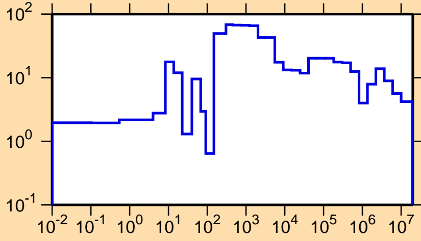
\Delta\sigma/\sigma vs. E for ^{112}\text{Te}(n,el.)
