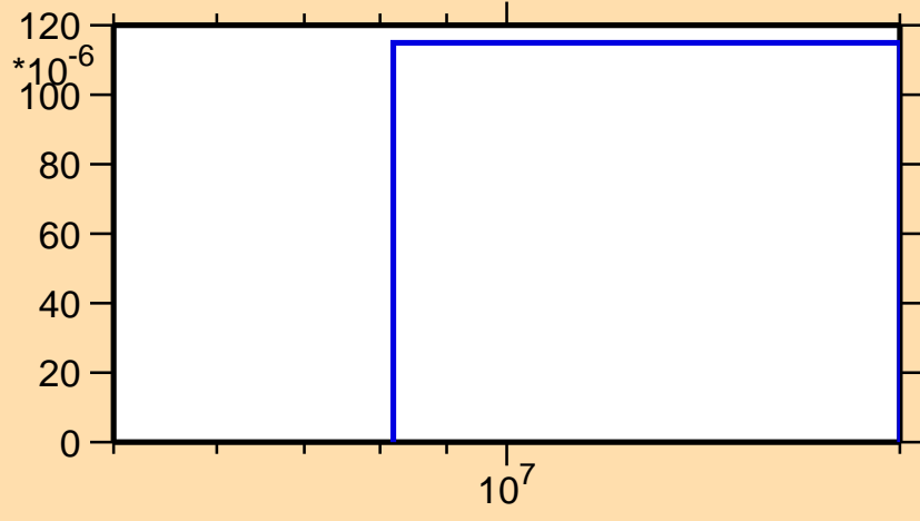
\sigma vs. E for ^{112}\text{Te}(n,t)
