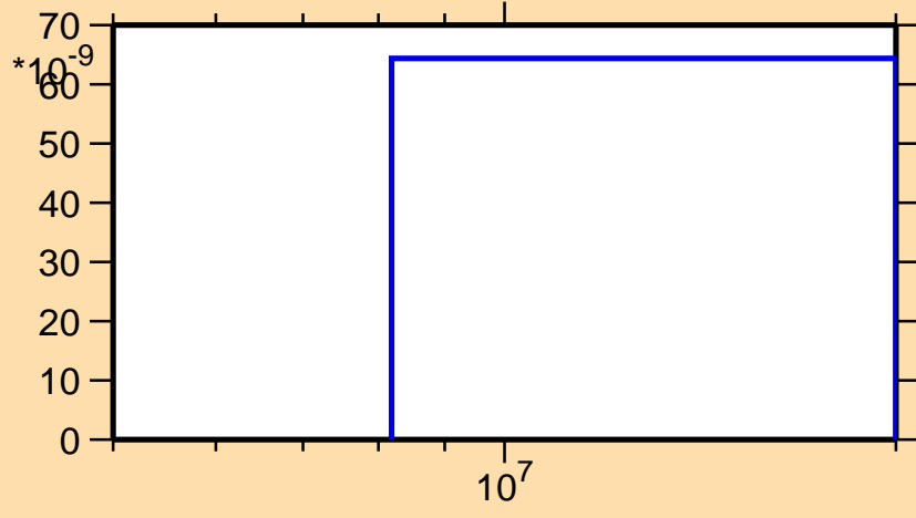
\sigma vs. E for ^{112}\text{Te}(n,2np)
