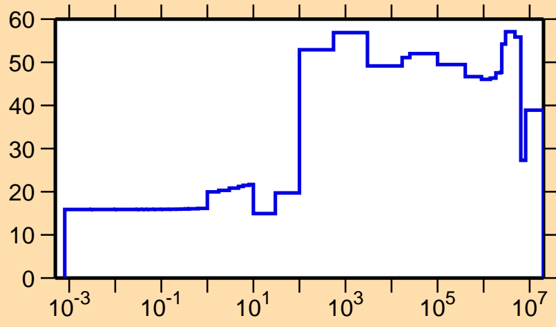
\Delta\sigma/\sigma vs. E for ^{112}\text{Te}(n,\gamma)
