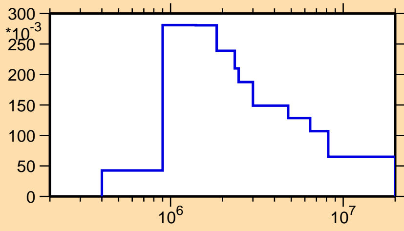
\sigma vs. E for ^{112}\text{Te}(n,n_1)
