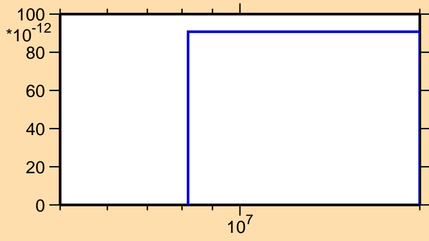
\sigma vs. E for ^{112}\text{Te}(\text{mt } 34)
