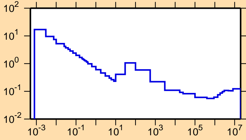
\sigma vs. E for ^{112}\text{Te}(n,\alpha)
