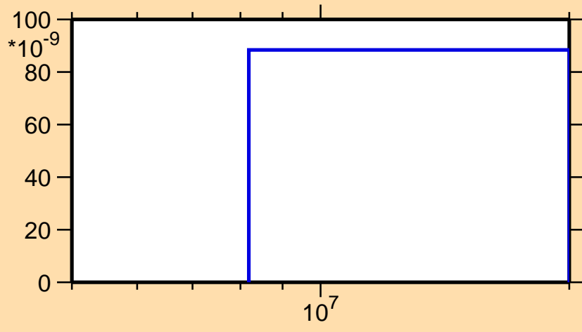
\sigma vs. E for ^{112}\text{Te}(n,\text{pt})
