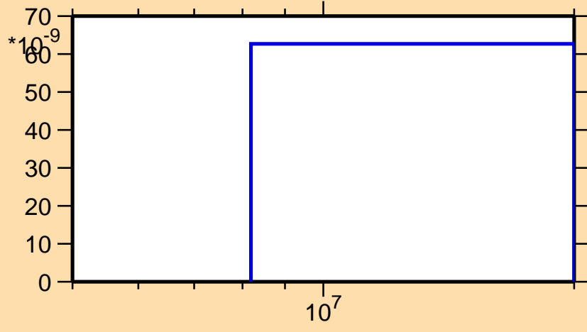
\sigma vs. E for ^{112}\text{Te}(n,2n\alpha)
