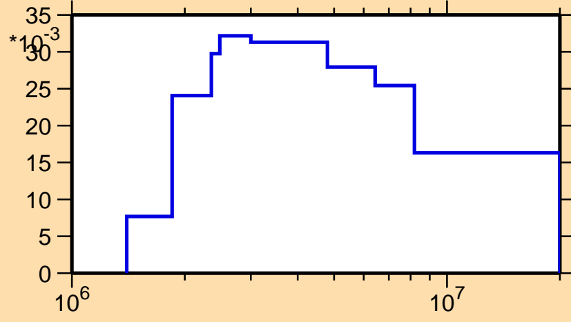
\sigma vs. E for ^{112}\text{Te}(n,n_2)
