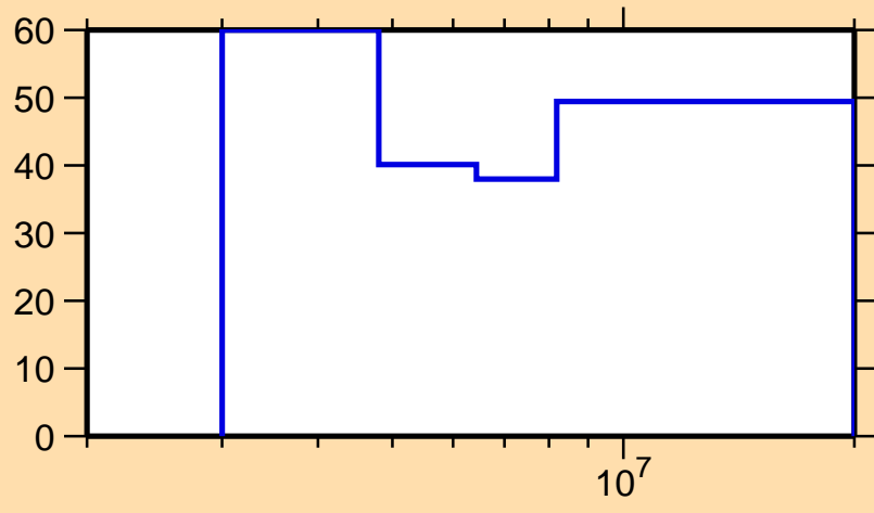
\Delta\sigma/\sigma vs. E for ^{114}\text{Te}(n,n\text{cont.})
