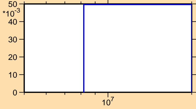
\sigma vs. E for ^{114}\text{Te}(n,2n)
