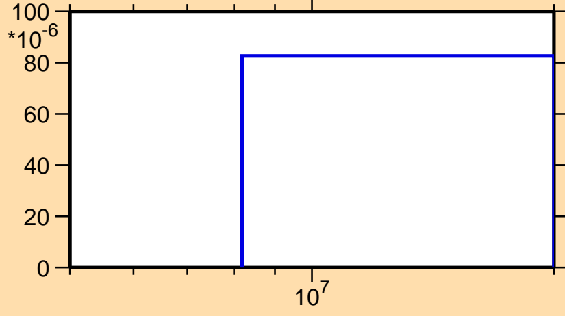
\sigma vs. E for ^{114}\text{Te}(n,t)
