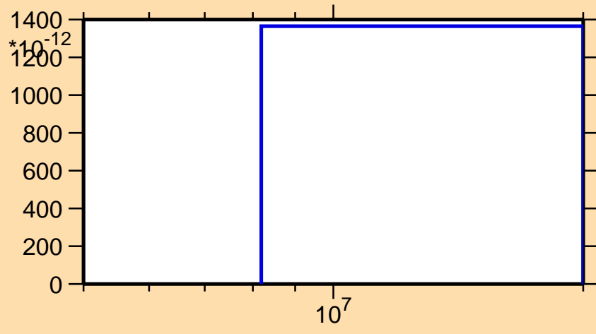
\sigma vs. E for ^{114}\text{Te}(n,\text{pt})
