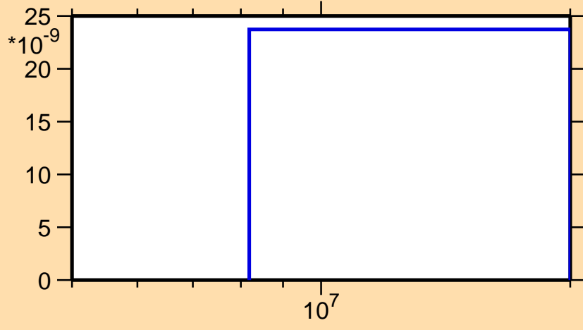
\sigma vs. E for ^{114}\text{Te} (mt 45)
