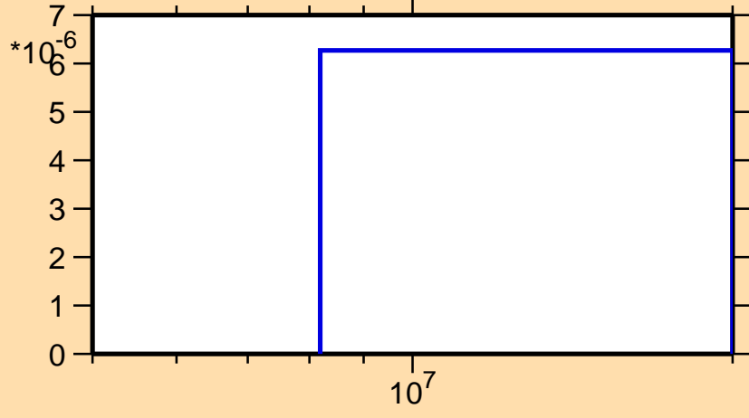
\sigma vs. E for ^{114}\text{Te}(n,pd)
