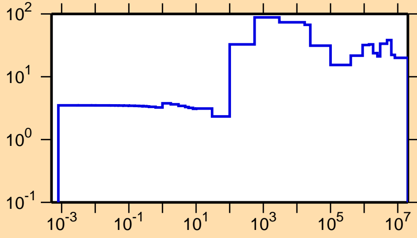
\Delta\sigma/\sigma vs. E for ^{114}\text{Te}(n,el.)
