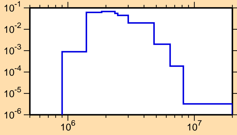
\sigma vs. E for ^{114}\text{Te}(n,n_3)
