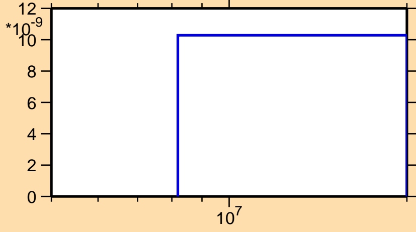
\sigma vs. E for ^{114}\text{Te}(n,\text{nd})
