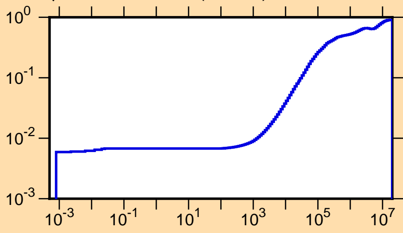
\mu vs. E for ^{115}\text{Te}(\text{mt251})
