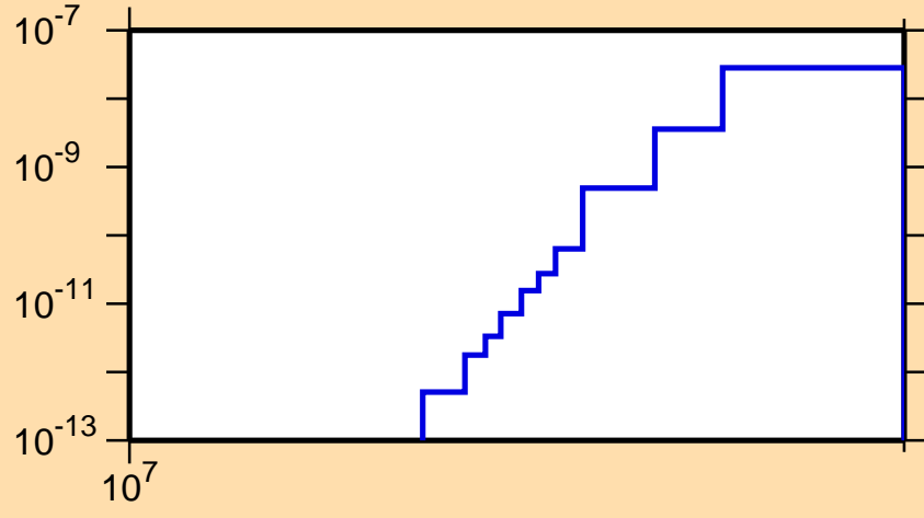
\sigma vs. E for ^{115}\text{Te}(\text{mt117})
