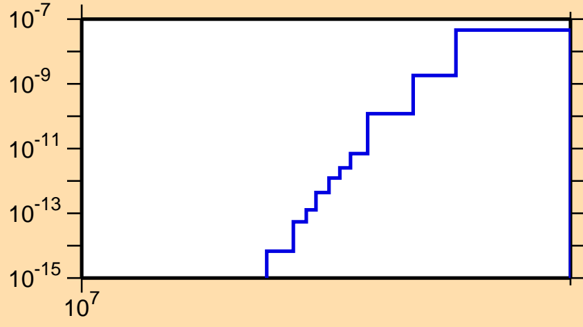
\sigma vs. E for ^{115}\text{Te} (mt 34)
