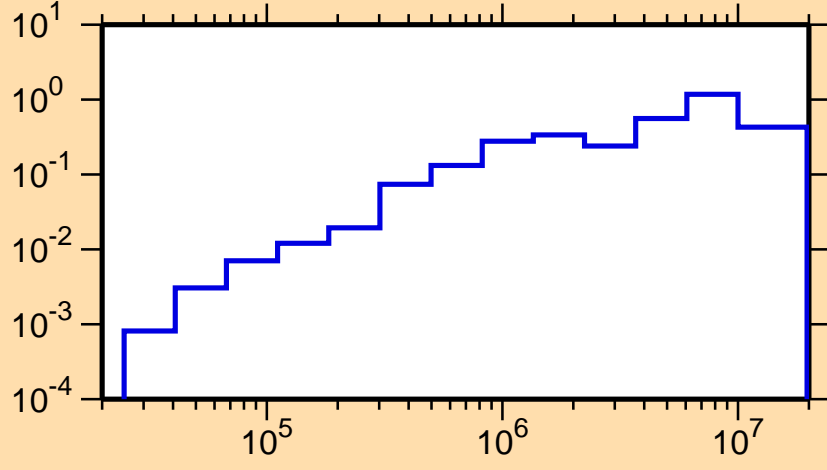
\sigma vs. E for ^{115}\text{Te}(n,\text{inel.})
