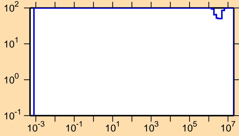
\Delta\sigma/\sigma vs. E for ^{115}\text{Te}(n,p)
