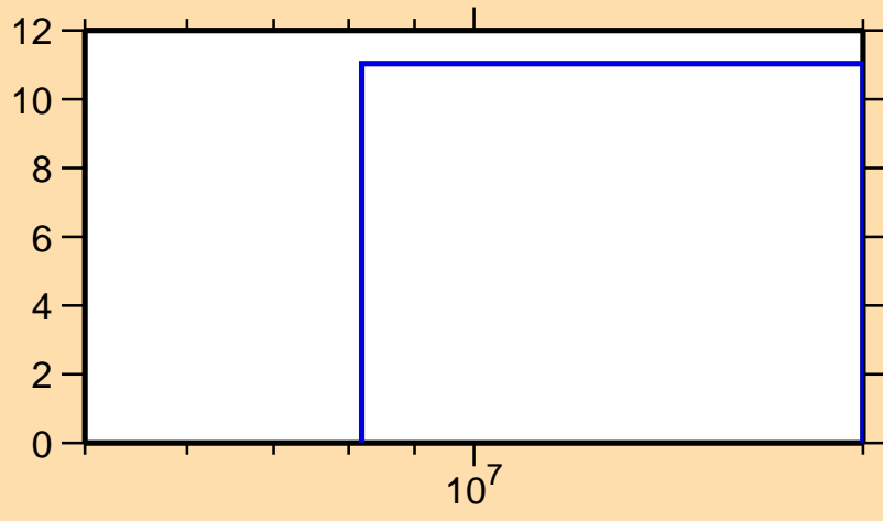
\Delta\sigma/\sigma vs. E for ^{115}\text{Te}(n,\text{tot.})
