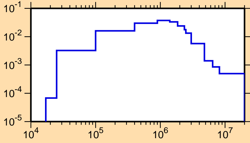
\sigma vs. E for ^{115}\text{Te}(n,n_1)
