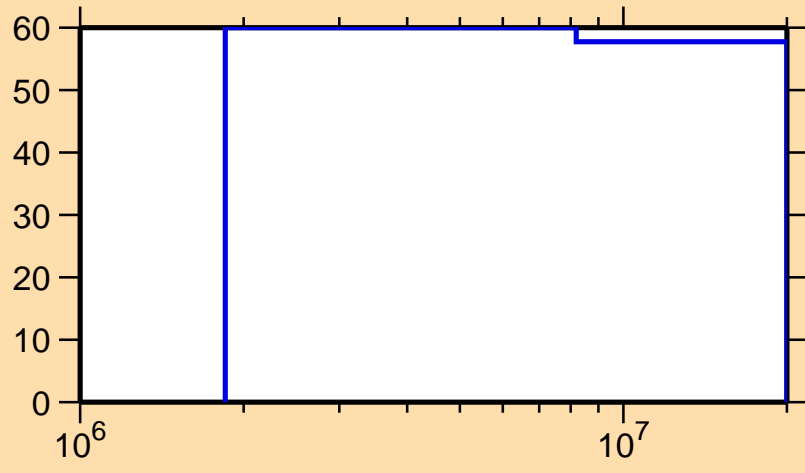
\Delta\sigma/\sigma vs. E for ^{115}\text{Te}(n,n\text{cont.})
