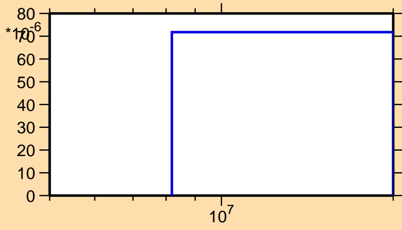
\sigma vs. E for ^{115}\text{Te}(n,2np)
