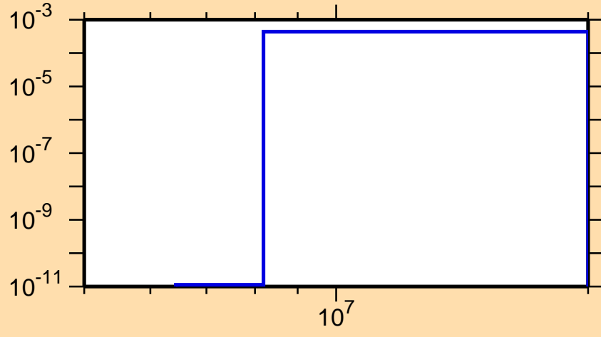
\sigma vs. E for ^{115}\text{Te}(n,t)
