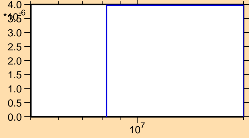
\sigma vs. E for ^{115}\text{Te}(n,pd)
