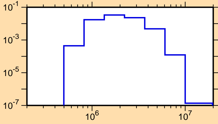
\sigma vs. E for ^{115}\text{Te}(n,n_3)
