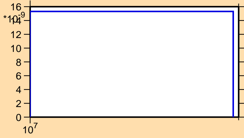
\sigma vs. E for ^{115}\text{Te} (mt 45)
