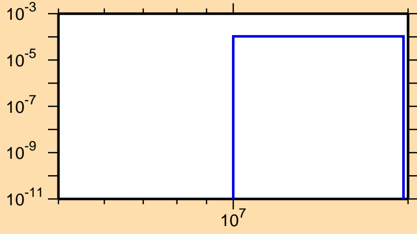
\sigma vs. E for ^{115}\text{Te}(n,2n\alpha)
