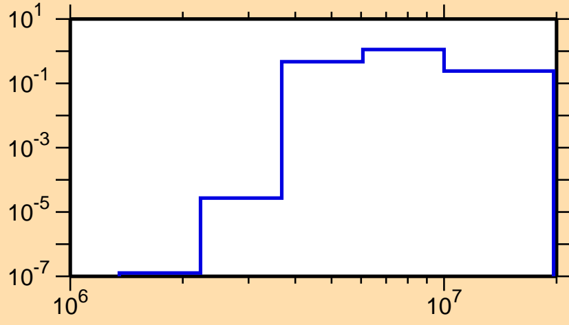
\sigma vs. E for ^{115}\text{Te}(n,n\text{cont.})
