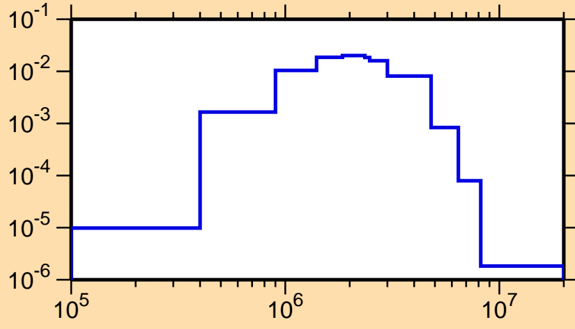
\sigma vs. E for ^{115}\text{Te}(n,n_2)
