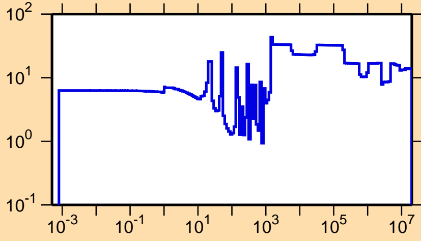
\Delta\sigma/\sigma vs. E for ^{116}\text{Te}(n,el.)
