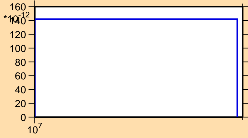
\sigma vs. E for ^{116}\text{Te} (mt 45)
