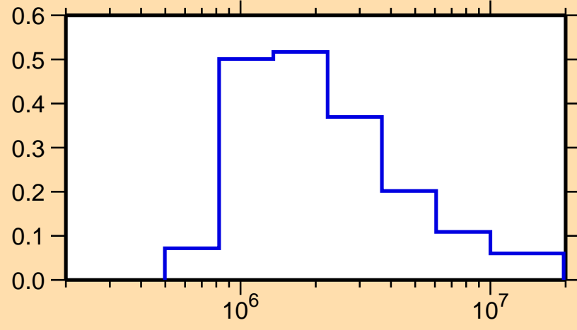
\sigma vs. E for ^{116}\text{Te}(n,n_1)
