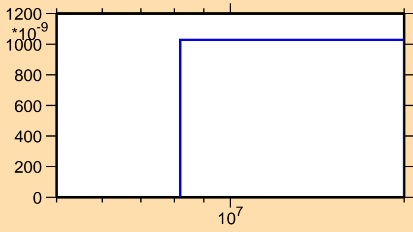
\sigma vs. E for ^{117}\text{Te}(n,\text{nd})
