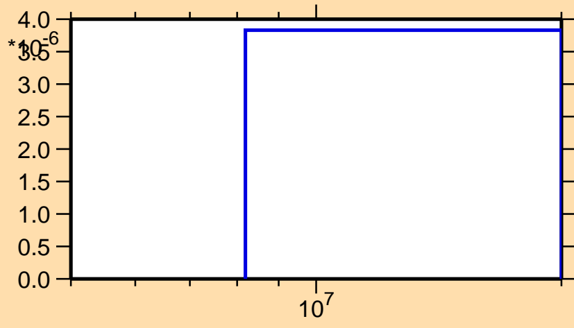
\sigma vs. E for ^{117}\text{Te}(n,\text{He}3)
