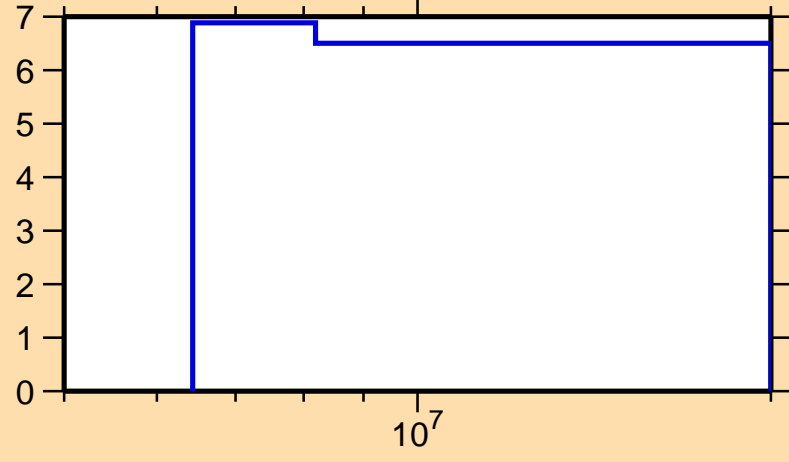
\Delta\sigma/\sigma vs. E for ^{117}\text{Te}(n,\text{tot.})
