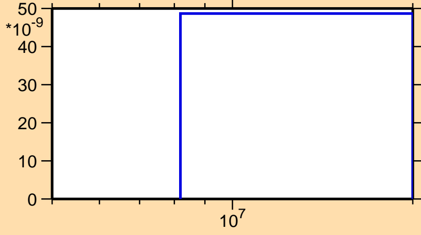
\sigma vs. E for ^{117}\text{Te}(n,pd)
