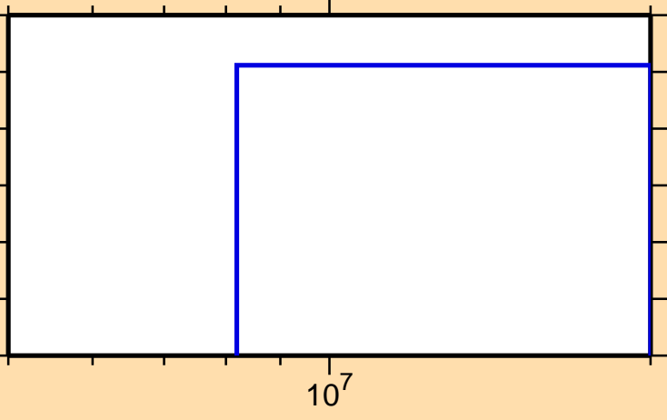
\sigma vs. E for ^{117}\text{Te}(n,3n)
