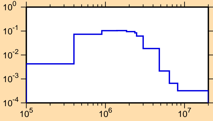
\sigma vs. E for ^{117}\text{Te}(n,n_2)
