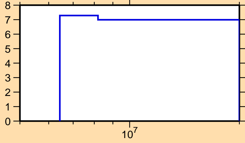
\Delta\sigma/\sigma vs. E for ^{117}\text{Te}(n,\text{nonel.})
