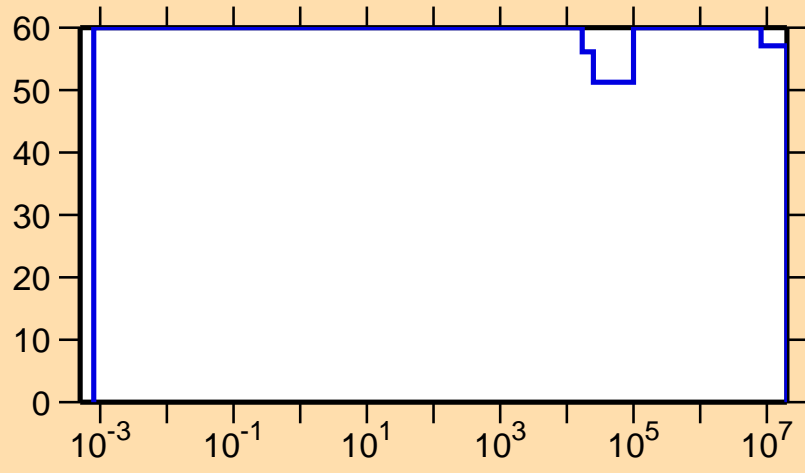
\Delta\sigma/\sigma vs. E for ^{117}\text{Te}(n,p)
