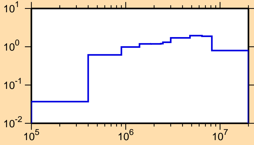
\sigma vs. E for ^{117}\text{Te}(n,\text{inel.})
