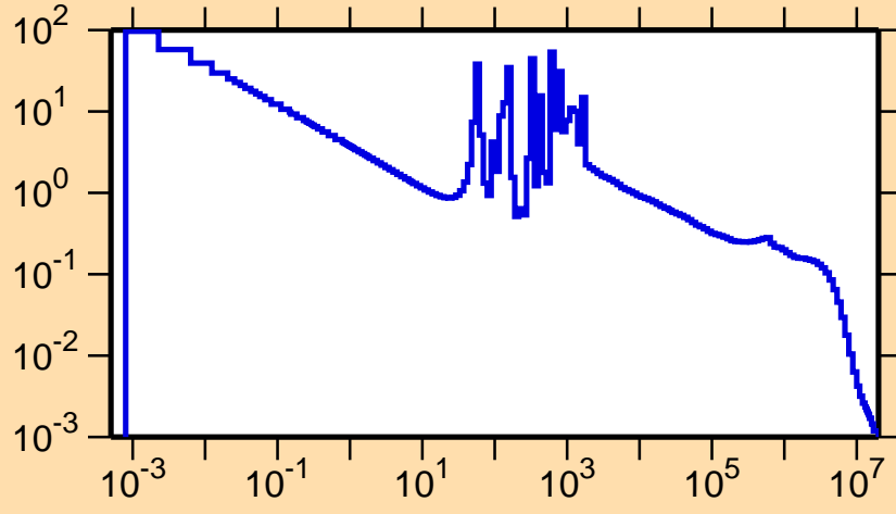
\sigma vs. E for ^{118}\text{Te}(n,\gamma)
